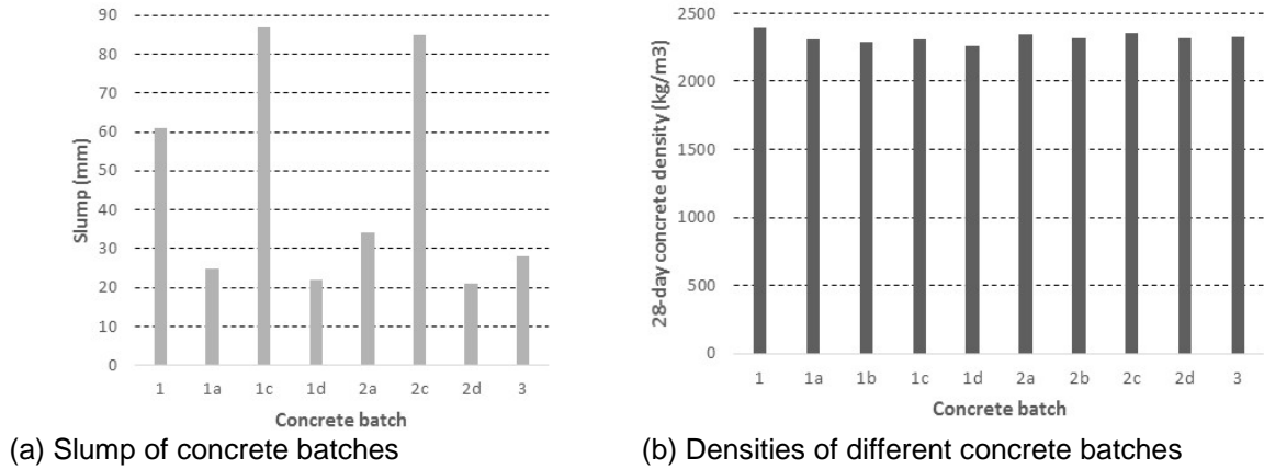
Fig. 6. Slump and density comparison among concrete batches
