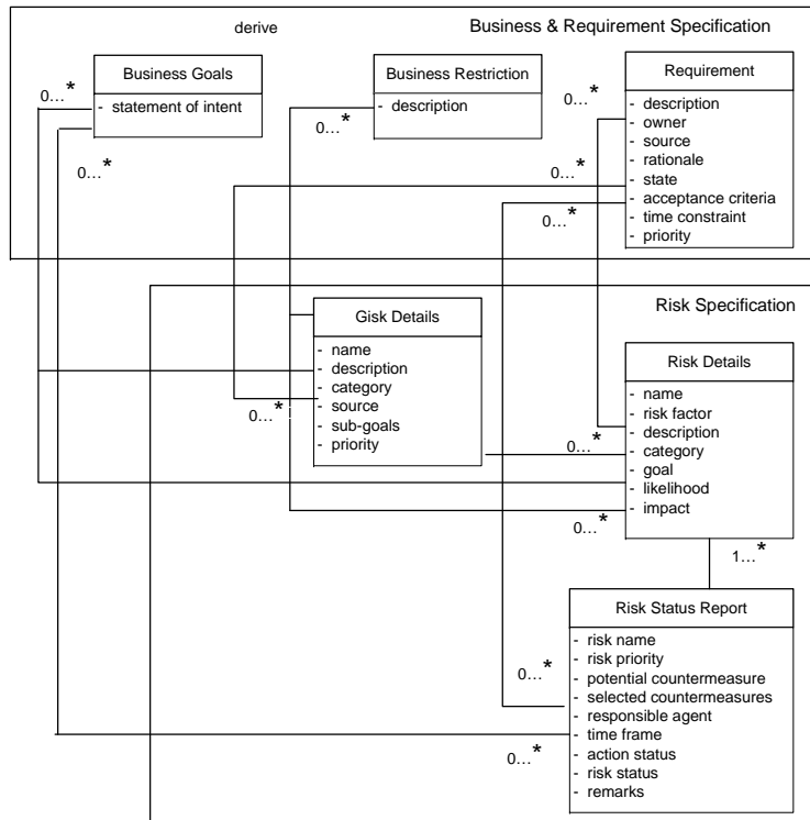
Figure 4: Attributes Dependency of Requirements and Risk Artefacts
