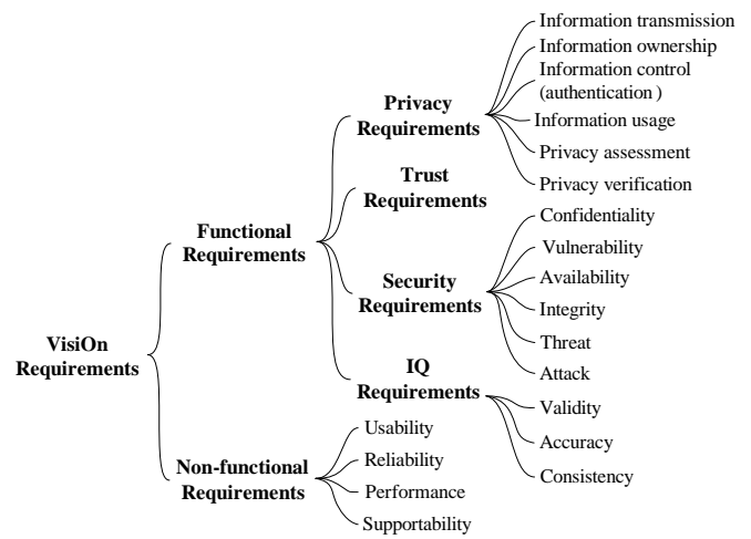
Fig. 6. VisiOn user requirements taxonomy
