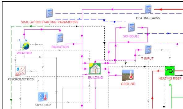
Figure 1 Extracted view of the Trnsys HVAC model
