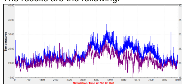
Figure 8 Apartment 1 internal monitored (violet line) and simulated (blue line) average temperature (°C).
