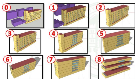
Figure 4 Building envelope simplification
