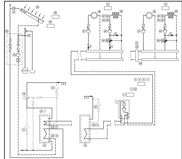
Figure 2 Sub-system A
