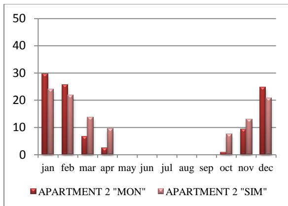
Figure 12 Apartment 2 monitored ("MON") and simulated ("SIM") monthly gas consumptions (m 3 ).
