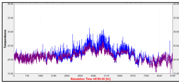
Figure 10 Apartment 3 internal monitored (violet line) and simulated (blue line) average temperature (°C).
