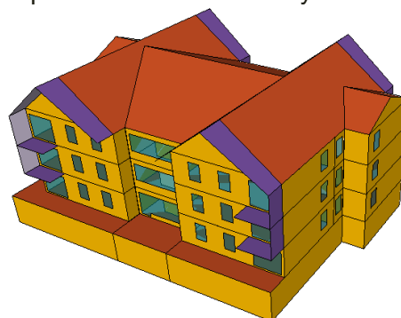
Figure 7 Complete model for building envelope (Trnsys3D)
