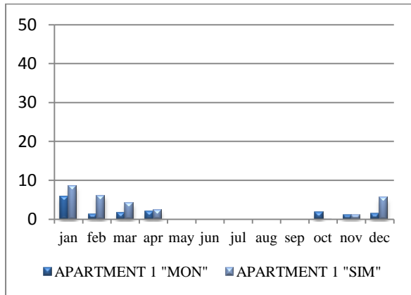
Figure 11 Apartment 1 monitored ("MON") and simulated ("SIM") monthly gas consumptions (m 3 ).
