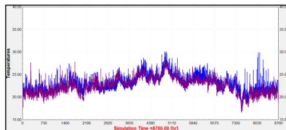
Figure 9 Apartment 2 internal monitored (violet line) and simulated (blue line) average temperature (°C).
