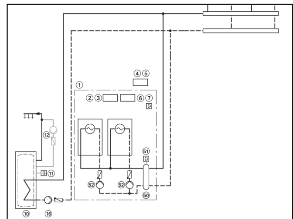
Figure 3 Sub-system B
