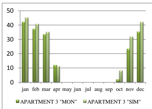
Figure 13 Apartment 3 monitored ("MON") and simulated ("SIM") monthly gas consumptions (m 3 ).
