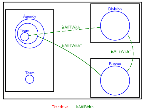
Figure 8. Transitive property
