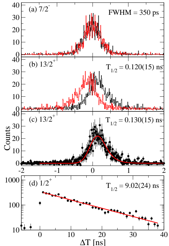
FIG. 4. (Colour Online) The forward (black) and reverse (red) time distributions for (a) the 896 keV state, obtained by gating on the 1547- and 896 keV coincidences and (b) the 1609 keV state, obtained by gating on the photo-peaks of the feeding (992- and 1132 keV) and de-exciting (1609 keV) transitions. The forward time profile of (c) the 1609 keV state using the same gates as in (b) and (d) the 2443 keV state, obtained by gating on the photo-peaks of the feeding (324- and 402 keV) and de-exciting (1547 keV) transitions.
