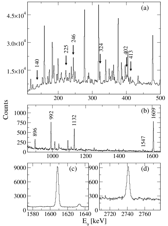
FIG. 2. The \gamma -ray energy spectra measured in the HPGe detectors: (a) The total projection of a ( E_\gamma - E_\gamma ) matrix, with the 140-, 225-, 246-, 324-, 402- and 413 keV 209 Bi transitions used as gates marked by arrows. (b) An energy spectrum created as a result of using the gates in panel (a), with the high-energy \gamma -ray transitions of interest in 209 Bi labelled with their energy. (c,d) show the cleanliness of the 1609- and 2741 keV transitions in the singles spectra, used for the angular distribution analysis.
