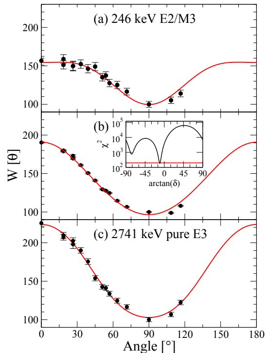
FIG. 5. (Colour Online) The \gamma -ray intensity as a function of angle for the (a) 246 mixed E2/M3 transition (b) 1609 keV transition and (c) 2741 keV pure E3 transition. The inset to (b) shows the \chi^2 value as a function of \arctan(\delta) .
