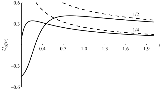
FIGURE 10. The plots of U_{eff(v)} versus \tilde{t} predicted by (3.17) (arbitrary \tilde{t} ; solid curves) and (4.9) (large \tilde{t} ; dashed curves) for b = 1/2 and 1/4 (numbers near the curves).
