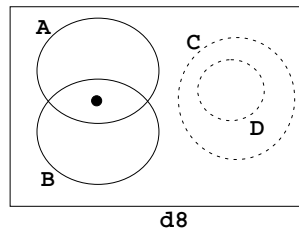
Fig. 4. Resultant, semantically equivalent, spider diagram.
