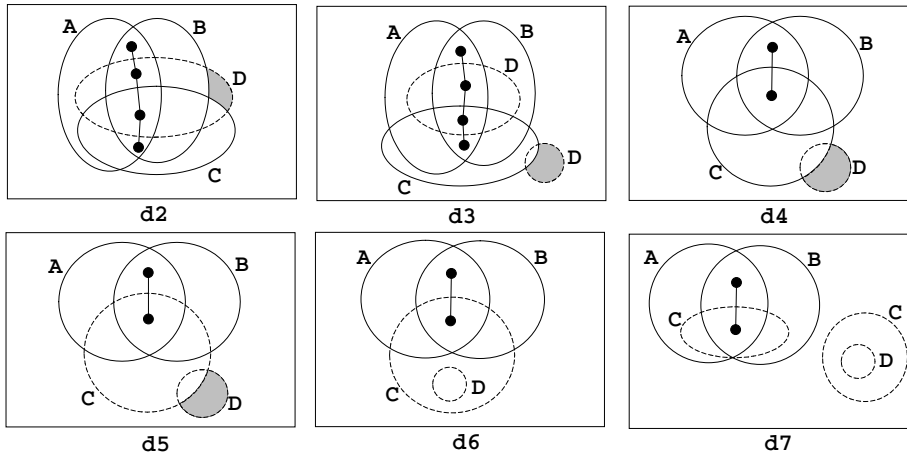
Fig. 3. Reasoning with projected contours.
