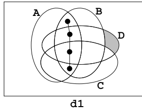
Fig. 2. Initial spider diagram.
