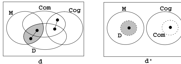
Fig. 1. Two semantically equivalent spider diagrams.
