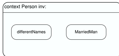
Fig. 13. Combining Constraints
