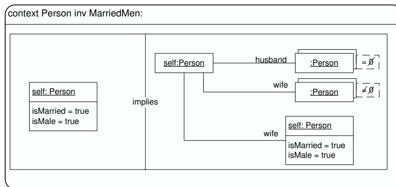
Fig. 11. Invariant 4: Married man have a wife and no husband
