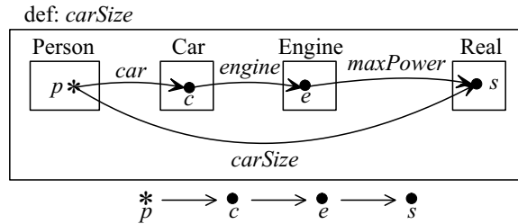
Fig. 3. Definition: carsize
