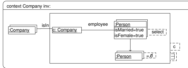
Fig. 10. Invariant 3: There is a company with no female married employees
