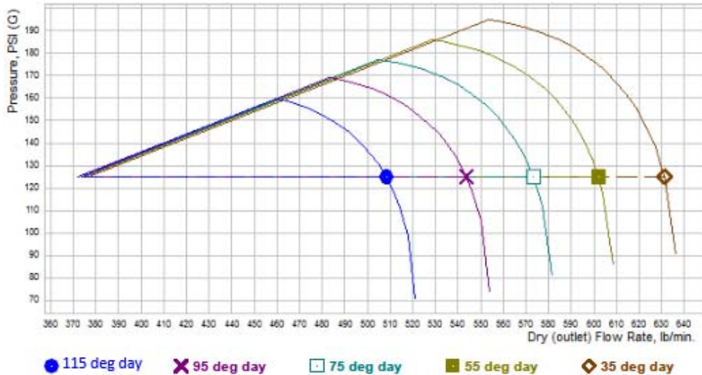
Figure 5. Pressure vs. Flow at Various Ambient Air Temperatures
