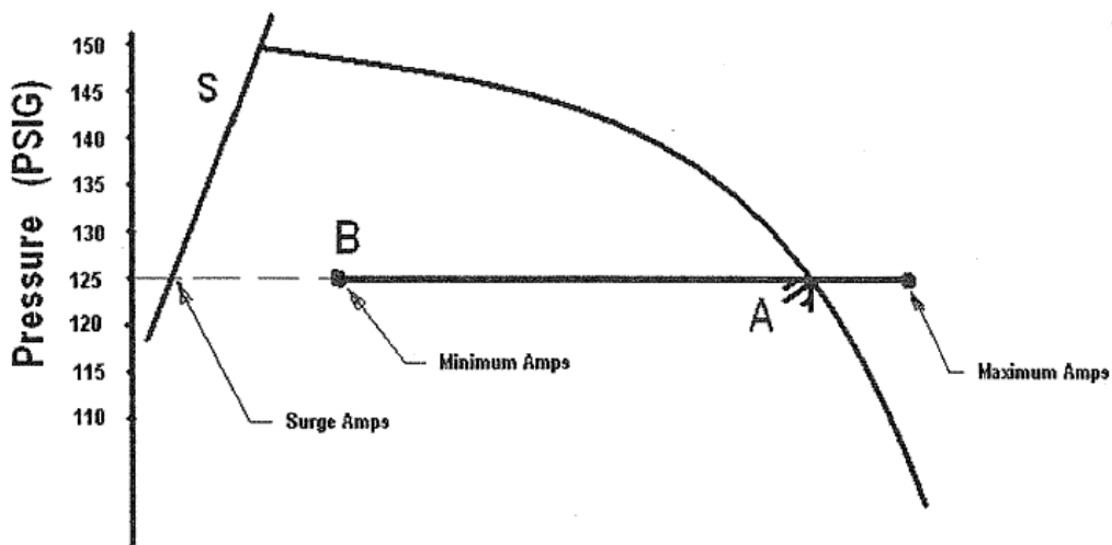
Figure 22. Suction Throttle Mode Compressor Control Curve
