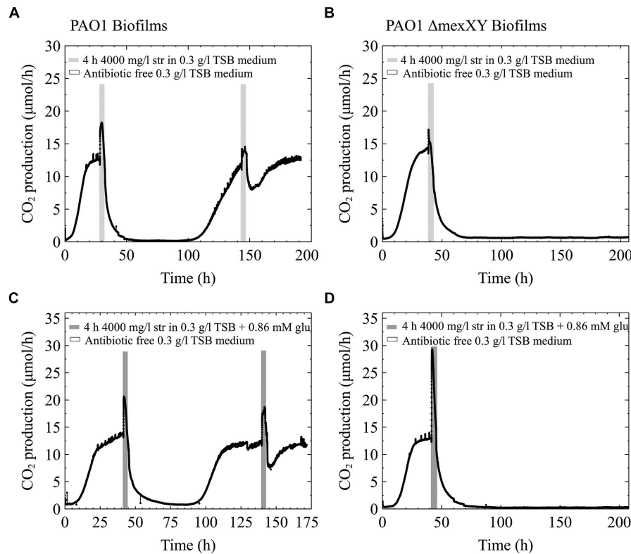
FIGURE 6 | Effect of inoculum – the experiments shown in Figure 5 were repeated, with the only exception that the cultures used for inoculation were first streak plated prior to growing overnight cultures. All other information as described in Figure 5.
