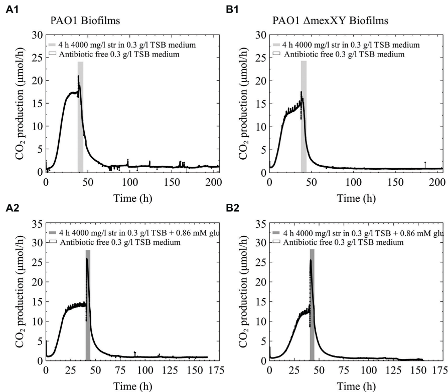
FIGURE 5 | CO 2 production (µmol/h) of biofilms of P. aeruginosa PAO1 (A) and PAO1 Δ mexXY (B) grown in 0.3 g/l TSB. The biofilms were grown for less than 48 h and had reached steady state CO 2 output before they were exposed to 4000 mg/l streptomycin for 4 h. (A1) and (B1) biofilms were exposed to streptomycin in 0.3 g/l TSB medium. (A2) and (B2) were exposed to streptomycin in 0.3 g/l TSB medium with the addition of 0.86 mM glucose (glu).
