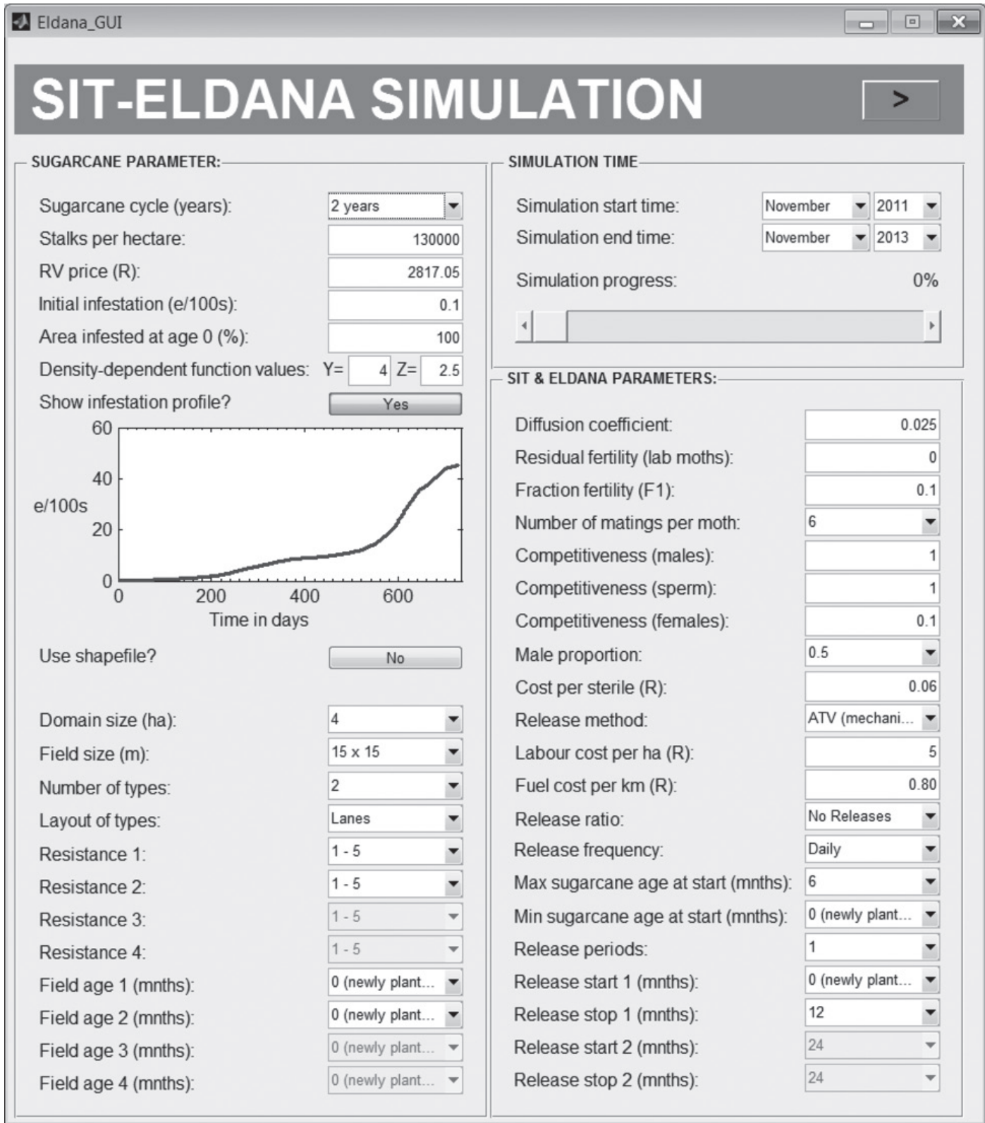
Fig. 6. The graphical user interface designed for the SIT/IS simulation tool for the field application of a SIT/IS strategy against Eldana saccharina in sugarcane. The initial infestation, e/100s, is the number of borers per 100 stalks of sugarcane.
