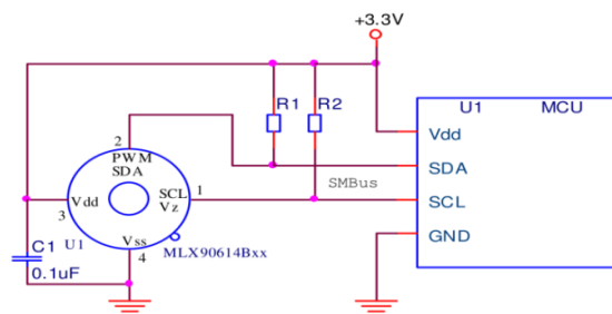
FIGURE 5: CIRCUIT DIAGRAM OF INFRARED THERMAL SENSOR (Mlx90614)
