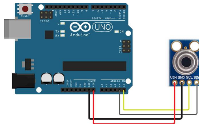
FIGURE 7: INTEGRATION OF MLX90614 IR THERMAL SENSOR WITH ARDUINO UNO (ATMEGA 328) BOARD
