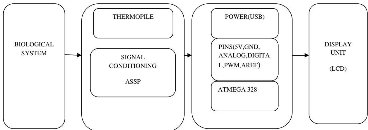
FIGURE 4: BLOCK DIAGRAM OF THE PROPOSED SYSTEM
