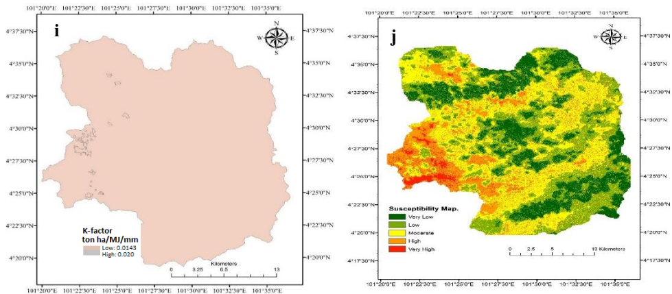
Fig. 1. (a) Inventory map (b) LS-factor (c) LineDen (d) DrainDen (e) SMI (f) LST (g) NDVI (h) R-factor (i) k-factor (j) Erosion susceptibility maps
