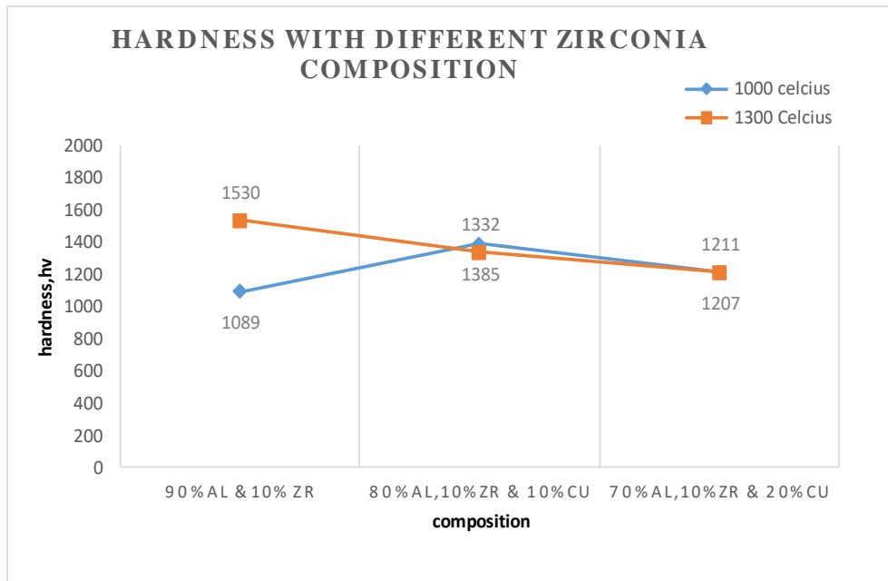
Figure 2. Hardness of samples with different composition and sintering temperature.
