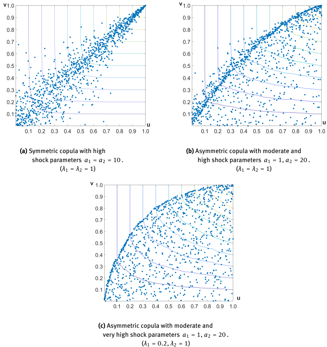
Figure 3: Scatter plots of copulas for different parameter settings based on samples of size 1000. The contour lines of the empirical copula functions for the values 0.1, \dots, 0.9 are also shown.
