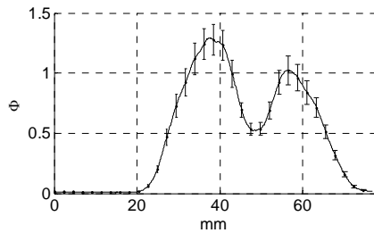
Figure 9: Average curve from 14 SLIPI measurements at 4 CAD ATDC corresponding to 14 700 individual cycles. The error bars indicate the standard deviation.
