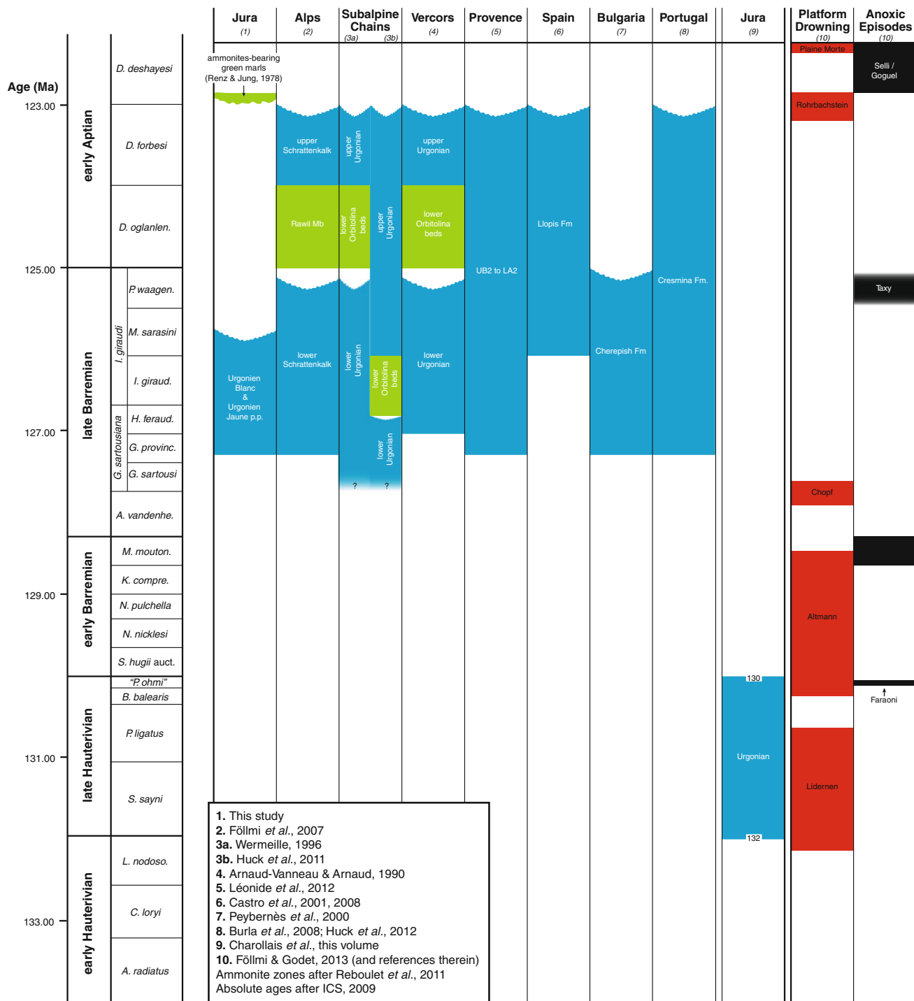
Fig. 2 Dating of Urganian-type limestone in various peri-Tethyan locations. Whereas its attribution to the late Barremian seems commonly agreed, a late Hauterivian age, as proposed by Charollais et al. (2013) is shifted by nearly 3 Ma
