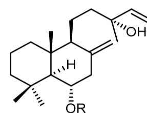
Fig. 2: Structure of the active compounds larixol (R=OH) and larixyl acetate (R=Ac)
