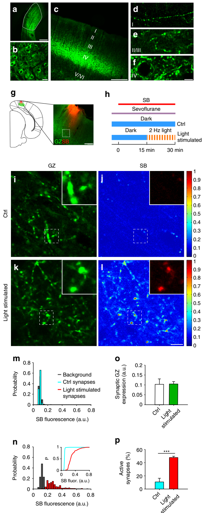
Fig. 4 Reporting the activation of thalamo-cortical synapses in vivo. a Visual thalamus (dLGN, dashed area) transduced by GZ lentiviral vector. b magnified view of transduced dLGN. c GZ-expressing synapses in V1 cortex. d–f Magnified views of layers I, II–III, and IV showing GZ-expressing presynaptic boutons. g Illustration (left) and merged fluorescent images (right) of the V1 cortex with sites of GZ expression (green) and SB injection (red; dashed square indicates a typical field for SB uptake analysis; see also Supplementary Figs. 6, 8). h Time flowchart showing SB perfusion, sevoflurane anesthesia, and dark or dark/light exposure visual stimuli. i–l V1 layer IV from control animals kept in the dark (Ctrl; i, j ) or exposed to light-pulses (light stimulated; k, l ), showing GZ expression ( i–k ) and SB uptake ( j–l ). Insets are magnified areas from dashed boxes. Color bars on the right are fluorescence LUTs. m, n SB fluorescence histograms for unstimulated control ( m ; cyan bars; N=233 synapses and N=93 neighboring non-GZ + areas, p_{ctrl-background}=0.45 , KS test) and light stimulated ( n ; red bars; N=177 synapses and N=92 neighboring non-GZ + areas, p_{light-background} < 0.0001 , KS test) GZ-expressing synapses, and for the corresponding background fluorescence (gray bars; same experiments as i–l ). Inset n , cumulative distributions of synaptic SB uptake for data set in m, n ( p_{light-ctrl} < 0.0001 , KS test). o, p Population data from control and light-stimulated animals for synaptic GZ expression ( o ; N=5 , p=0.93 ; two-samples permutation test) and activity ( p ; N=5 , p < 0.005 ; two-samples permutation test). Scale bars: 245 \mu\text{m} ( a, c, g ), 10 \mu\text{m} ( b, d–f, i–l )
