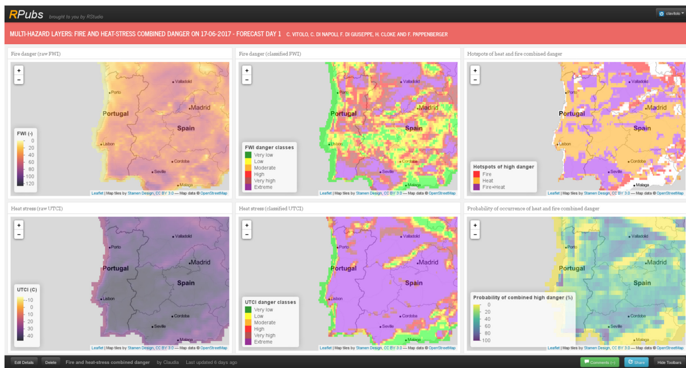
Fig. 9. Web-application to explore sample multi-hazard layers: raw FWI rating (top left panel), raw UTCI (bottom left), reclassified FWI (top center) and UTCI (bottom center), map of forecasted hotspots (top right) and map of probability of occurrence of two concurring hazards (bottom right). The layers have been computed at pan-European scale, although the panels above zoom in to show Portugal and part of Spain.
