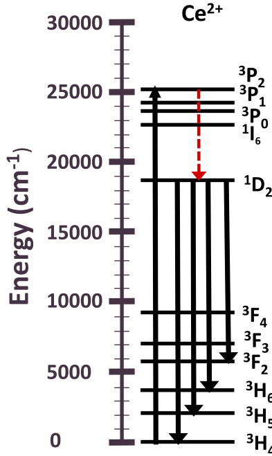
Figure 2. The proposed energy transfer mechanism for Ce^{2+} in Ce-doped fiber.
