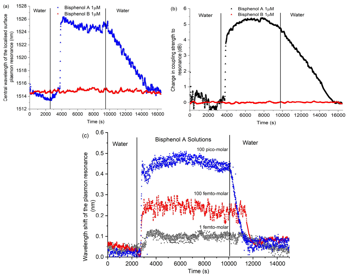
Figure 7 Typical examples of the wavelength shift response of the plasmonic sensors using the flow cell, showing association and dissociation of the bisphenol A with the aptamer, the biosensor results for both wavelength shift (a) and the change in optical strength (b) with a 1 \mu M solution. (c) Typical results with various bisphenol A solutions with differing concentrations: 1 fM ( \blacktriangle ), 100 fM ( \bullet ) and 100 pM ( \blacklozenge ).
