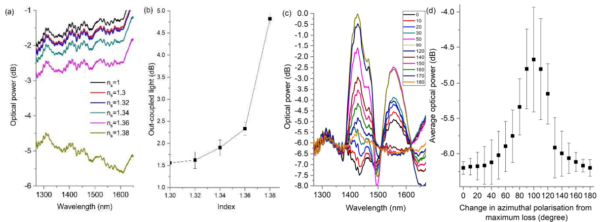
Figure 3. Typical refractive index (a,b) and polarisation (c, d) spectral properties of the D-shaped fibre used to fabricate the LSP sensors. (a) transmission spectrum and (b) spectral sensitivity with respect to refractive index of the surrounding medium (c) transmission spectrum and (d) spectral sensitivity with respect to the change in azimuthal polarisation of the illuminating light with maximum of coupling at 0 degree of the azimuthal polarisation.
