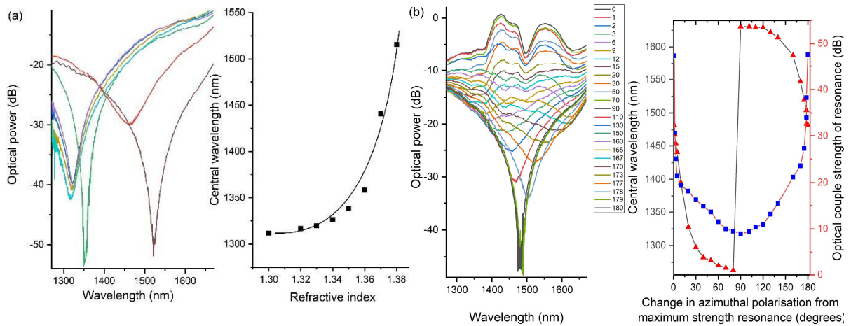
Figure 6 Typical refractive index and polarisation spectral properties of the D-shaped fibre after multi-layered coating and UV processing to produce the LSP sensing platform. (a) Transmission spectrum and spectral sensitivity with respect to refractive index of the surrounding medium with a maximum of coupling strength in air (b) Transmission spectrum and spectral sensitivity with respect to the change in azimuthal polarisation of the illuminating light with maximum of coupling at 0 degree of the azimuthal polarisation.
