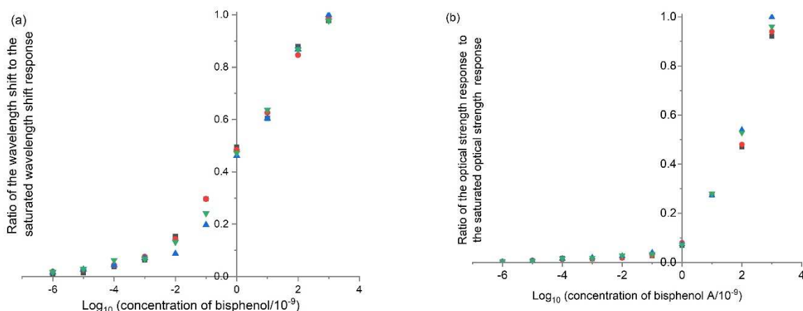
Figure 9 Concentration-response curves based upon (a) wavelength shifts and (b) optical strength changes for bisphenol A concentrations.
