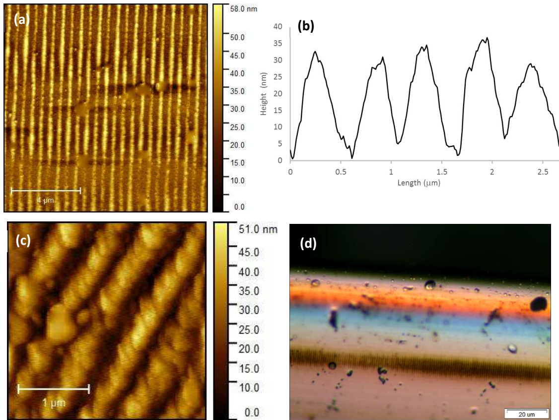
Figure 5 Typical surface profiles and images of the LSP sensor, (a) AFM image of the flat of the D-shaped UV processed coated fibre and the repeatable fabricated structure. (b) Line profile of an AFM image showing the cross-sectional view of the corrugation created on the surface. (c) High resolution AFM image of the UV processed surface. (d) optical microscope image of the flat of the D-shaped fibre showing the surface corrugation.
