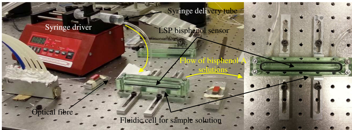
Figure 2. Image of the handling and solution sample delivery system.
