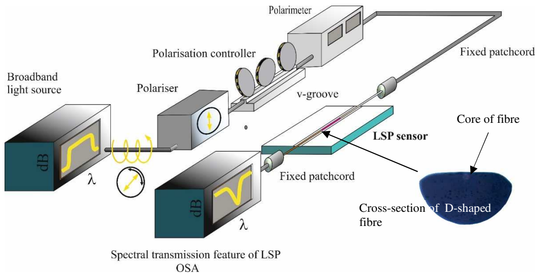
Figure 1 The characterisation apparatus for the LSP sensors.
