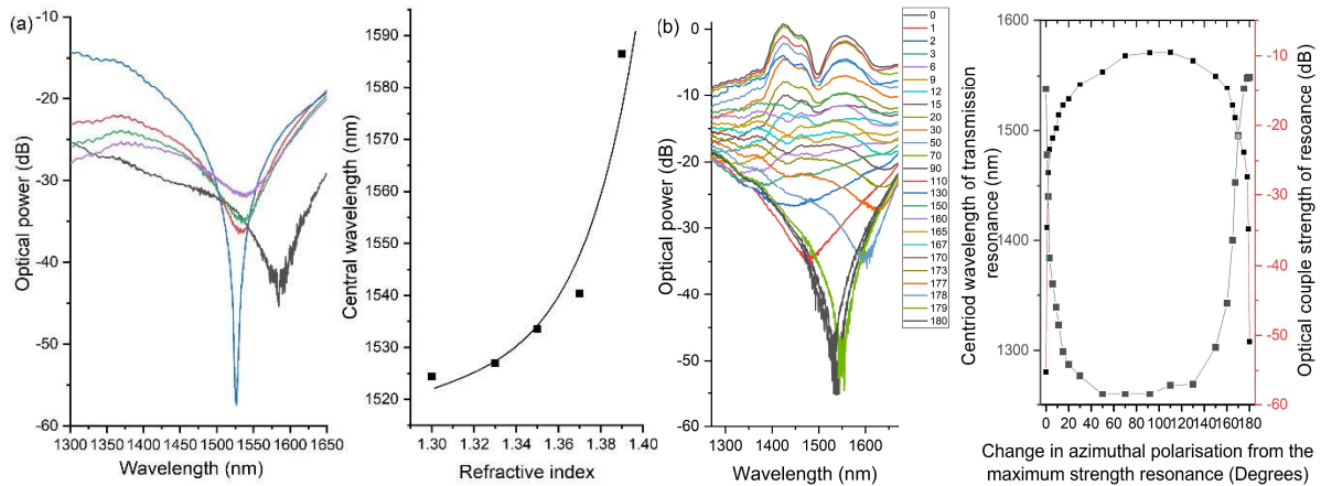
Figure 4. Typical refractive index and polarisation spectral properties of the D-shaped fibre with a multi-layered coating consisting of germanium, silicon dioxide and gold with thicknesses of 36nm, 24nm and 22nm respectively, used to fabricate the LSP sensors. (a) transmission spectrum and spectral sensitivity with respect to refractive index of the surrounding medium with a maxima of coupling strength in air (b) transmission spectrum and spectral sensitivity with respect to the change in azimuthal polarisation of the illuminating light with maximum of coupling at 0 degree of the azimuthal polarisation.
