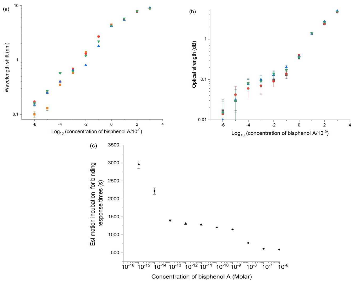
Figure 8. Spectral sensitivity of aptamer-coated, multilayered LSP fibre devices. (a) wavelength shifts as a function of bisphenol A concentration. (b) Change in optical coupling strength as a function of bisphenol A concentration. In figures (a) & (b), ●, ▲, ▼ and ■ represent measurements made with four different devices. (c) Estimation of incubation times of the binding reaction as a function of bisphenol A concentration obtained from four different devices over 12 experimental trials, the associated errors are the standard deviations calculated for each experiment at each concentration.
