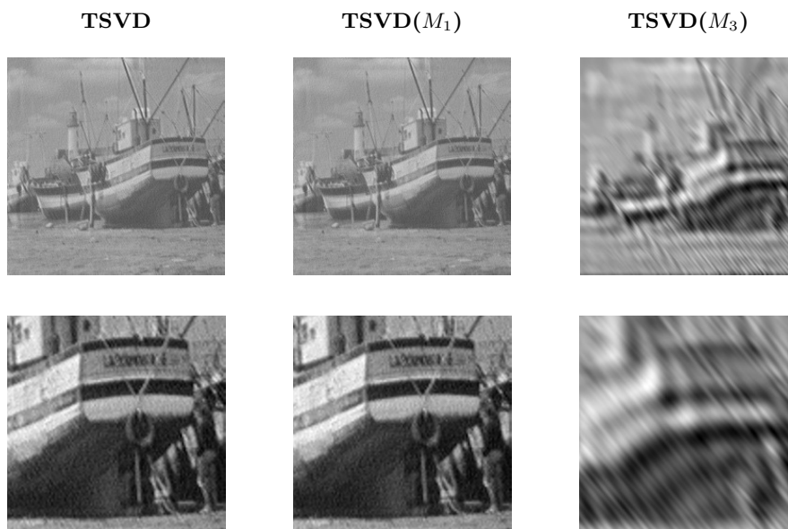
FIG. 6.7. The lower row displays blow-ups (200%) of the restored images in the upper row. From left to right: unpreconditioned Arnoldi-TSVD method ( 1.0481e - 01 , k = 26 ); TSVD( M_1 ) method ( 1.0081e - 01 , k_P = 50 , k = 7 ); TSVD( M_3 ) method ( 2.5948e - 01 , k_P = 50 , k = 35 ).
