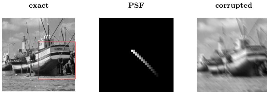
FIG. 6.5. Image deblurring problem with anisotropic motion blur. The upper row displays the test data. The lower row displays the best reconstructions obtained by: GMRES method ( 6.0804e-01 , k = 13 ); GMRES( C_1 ) method ( 1.6452e-01 , k = 2 ); GMRES( C_2 ) method ( 8.8234e-02 , k = 3 ); GMRES( C_3 ) method ( 6.0316e-01 , k = 3 ).
