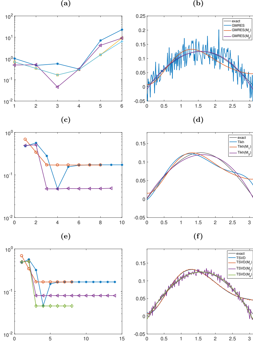
FIG. 6.1. Test problem baart , with m = 200 and \|\mathbf{e}\|/\|\mathbf{b}\| = 10^{-2} . (a) Relative error history, without any additional regularization and k_P = 9 . (b) Best approximations, without any additional regularization and k_P = 9 . (c) Relative error history, with Arnoldi-Tikhonov and k_P = 9 . (d) Approximations for k = 6 , with Arnoldi-Tikhonov and k_P = 9 . (e) Relative error history, with Arnoldi-TSVD and k_P = 39 . (f) Approximations for k = 9 , with Arnoldi-TSVD and k_P = 39 .
