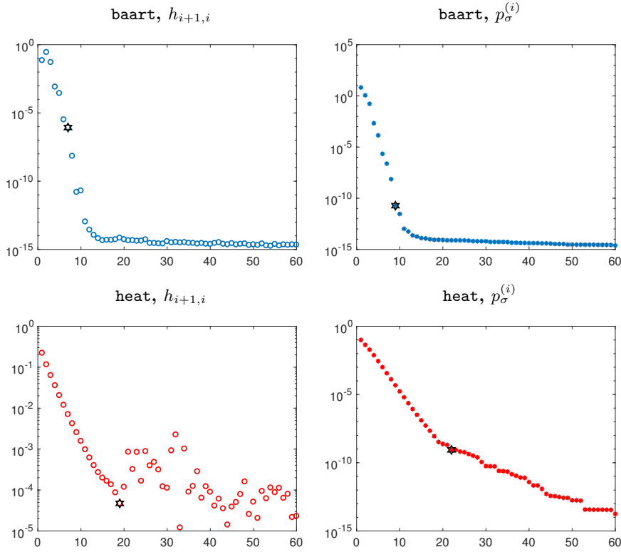
FIG. 6.3. Illustration of the stopping criteria (5.6) and (5.7) for the test problems baart (top row) and heat (bottom row). In the left column, the values of the subdiagonal entries h_{i+1,i} of the Hessenberg matrix H_{k+1,k} are plotted against i ( i = 1, \dots, k ). In the right column, the products p_{\sigma}^{(i)} := \sigma_1^{(i)} \sigma_{i+1}^{(i+1)} of the extremal singular values of H_{i+1,i} are plotted against i .
