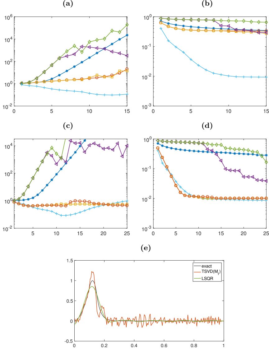
FIG. 6.2. Test problem heat , with m = 200 and \|\mathbf{e}\|/\|\mathbf{b}\| = 10^{-2} . (a) Relative error history, with Arnoldi-TSVD and k_P = 23 . (b) Relative residual history, with Arnoldi-TSVD and k_P = 23 . (c) Relative error history, with Arnoldi-Tikhonov and k_P = 60 . (d) Relative residual history, with Arnoldi-Tikhonov and k_P = 60 . (e) Best approximations, with Arnoldi-Tikhonov and k_P = 60 .
