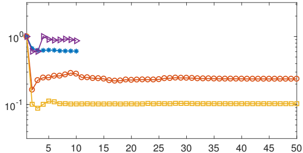
FIG. 6.4. Image deblurring problem with anisotropic motion blur. Relative error history of GMRES and right-preconditioned GMRES methods (with preconditioners C_1 , C_2 , and C_3 ). The GMRES and GMRES( C_3 ) curves are truncated because severe “semi-convergence” occurs.
