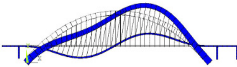
c) 2nd mode (vertical view): 0.4496 Hz
