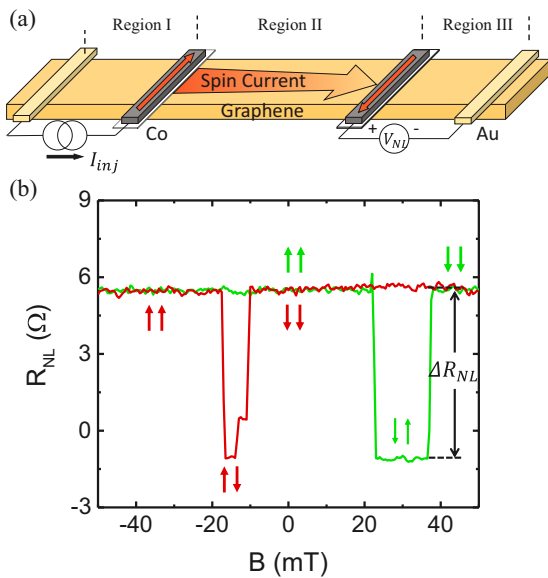
FIG. 1. (a) Schematic diagram of a graphene LSV and the non-local measurement geometry. An ac + dc current is applied on the left Co electrode to perform the bias-dependent spin injection study. Regions I, II, and III are corresponding to the spin injection, diffusion, and detection channel. (b) Typical nonlocal measurement data on a graphene lateral spin valve.
