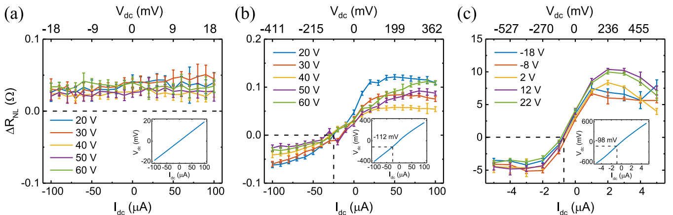
FIG. 4. Bias dependence of \Delta R_{NL} for graphene lateral spin valves with (a) transparent contacts ( V_{CNP} = 44 V), (b) MgO tunnel barrier contact with low contact resistance ( V_{CNP} = 45 V), and (c) MgO tunnel barrier contact with high contact resistance ( V_{CNP} = 2 V). The inset shows the IV curves integrated from the three-probe dV/dI measurement. The dashed lines in the inset show the position of I_{rev} and V_{rev} for the corresponding contacts.
