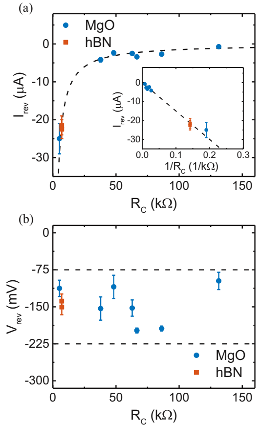
FIG. 5. (a) The reversal bias current ( I_{\text{rev}} ) plotted as function of contact resistance. Each data point represents a different injector electrode. The error bars represent the variation of I_{\text{rev}} with back-gate voltage. The dashed line plotted as I = -\frac{150 \text{ mV}}{R} is a guide to the eye. Inset: I_{\text{rev}} plotted as a function of 1/R_c , showing a linear dependence. (b) The reversal bias voltage ( V_{\text{rev}} ) plotted as function of contact resistance. All the reversal bias voltages are within the range between -75 and -225 mV, as indicated by the dashed lines.
