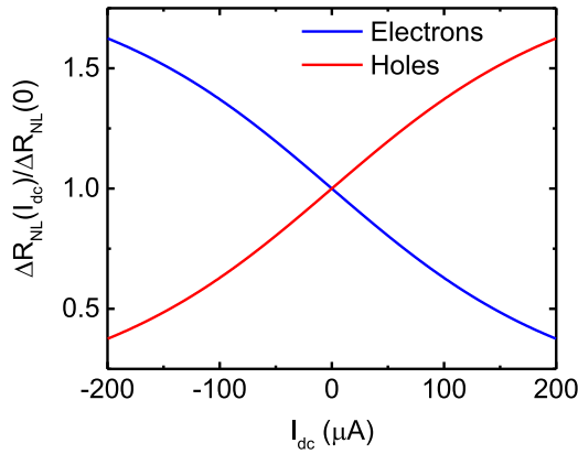
FIG. 6. Bias-dependent \Delta R_{\text{NL}}(I_{\text{dc}}) simulated with device parameters from typical graphene LSVs in this work, with \mu = 4000 \text{ cm}^2/\text{V s} , \lambda = 4 \text{ }\mu\text{m} , R_{\text{sq}} = 1 \text{ k}\Omega , D = 0.02 \text{ m}^2/\text{s} , and w = 1 \text{ }\mu\text{m} . The simulations are performed for both electron and hole dominated channel.
