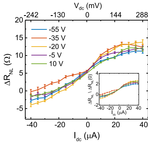
FIG. 3. Bias-dependent \Delta R_{NL} measured on a graphene LSV with hBN tunnel barrier at different back-gate voltage. The inset shows the normalized data. V_{CNP} = -27 V for this device.
