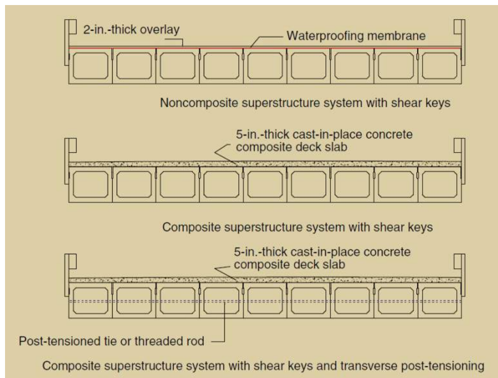
Figure 2.10: Various Practices in Adjacent Box Girder Bridge Design and Details (retrieved from Hanna et al., 2009)
