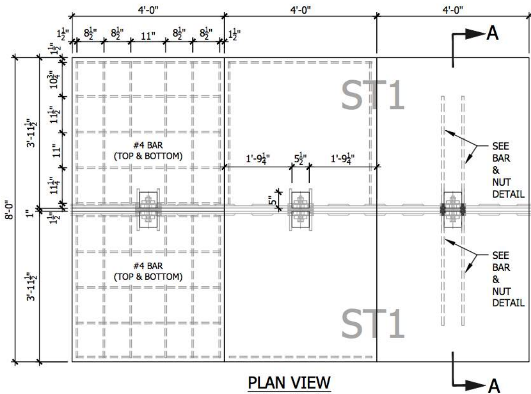
(a) rebar layout
