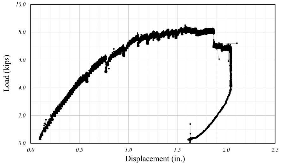
Figure 3.15: Load-Displacement Curve (Specimen F-F-1)
