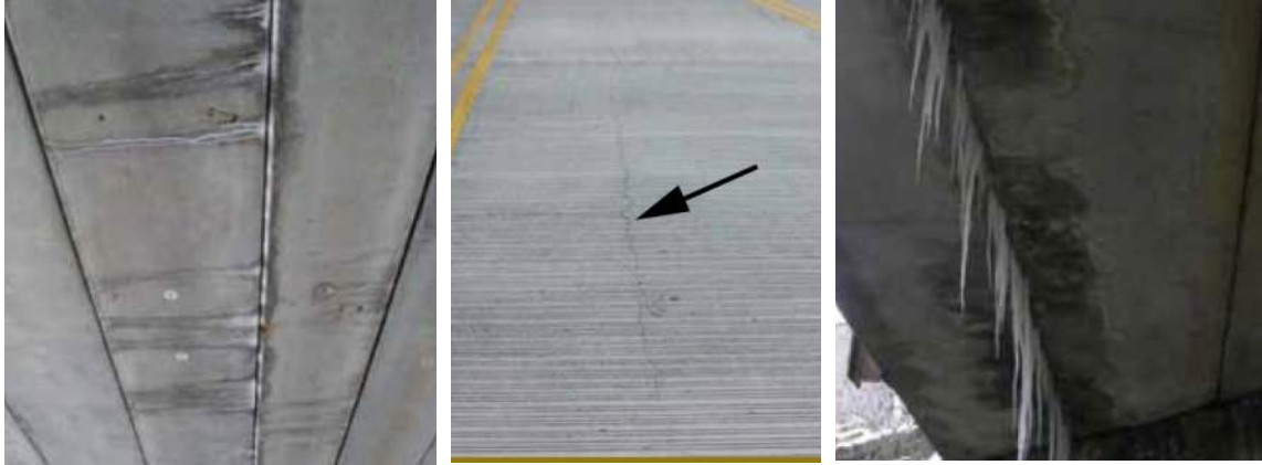
Figure 2.11: Major Problems Reported in Adjacent Beam Bridges: Longitudinal Crack along the Joint and Water and Chloride Penetration (retrieved from Russell, 2011)
