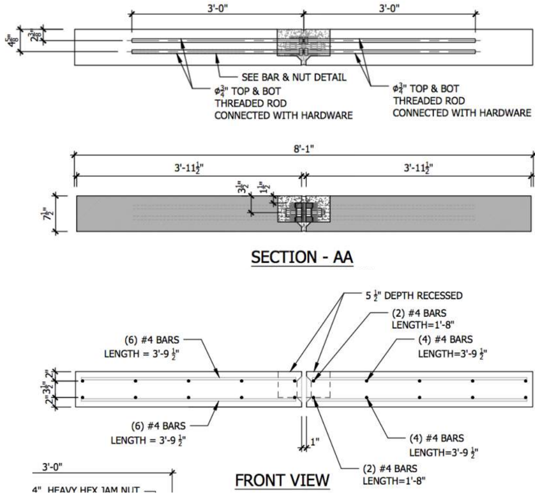
Figure 3.2: Plan and Section View of Slab Specimens Connected
