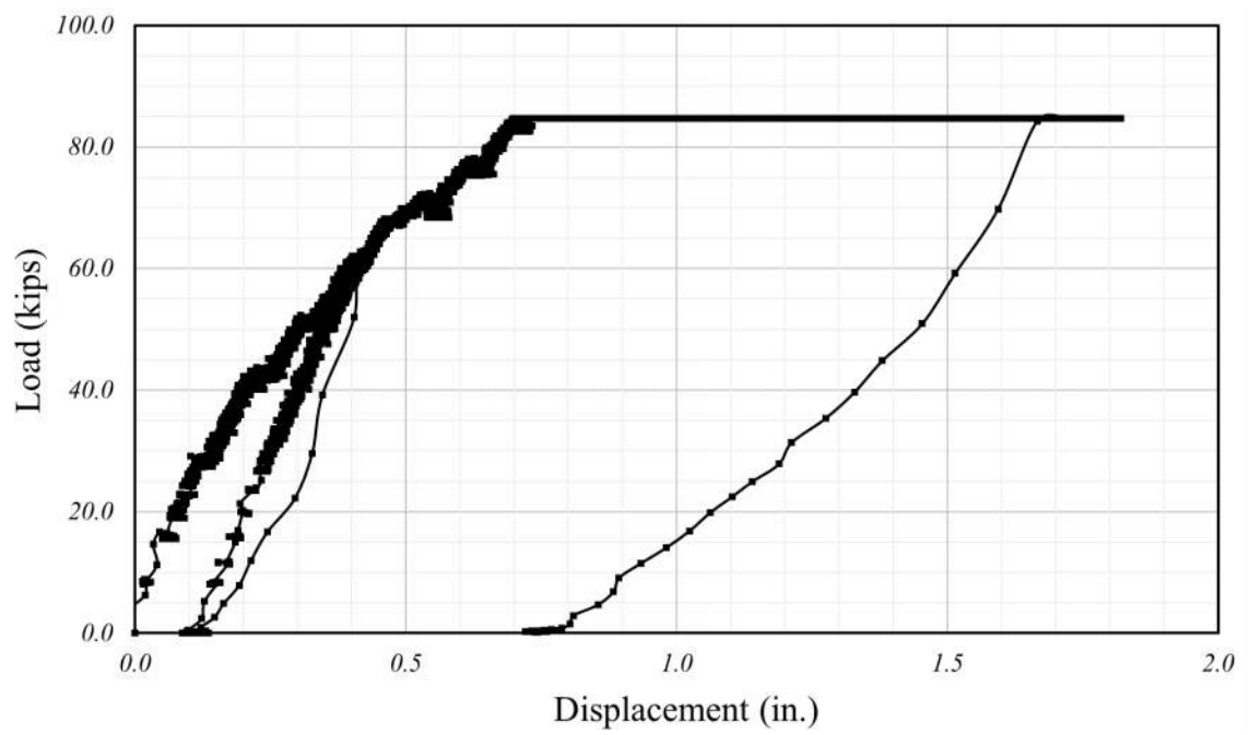
Figure 4.20: Load-Displacement of Specimen F-UHPC
