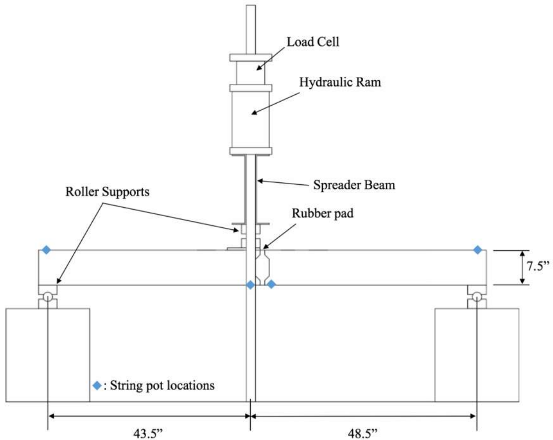
Figure 3.10: Three-Point Bending Test Setup
