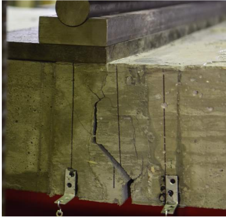
Figure 3.38: Grout Joint Close-up Photo (Specimen F-F-2, South view)
