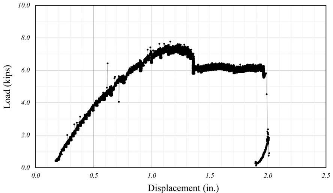
Figure 3.29: Load-Displacement Curve (Specimen C-F-1)
