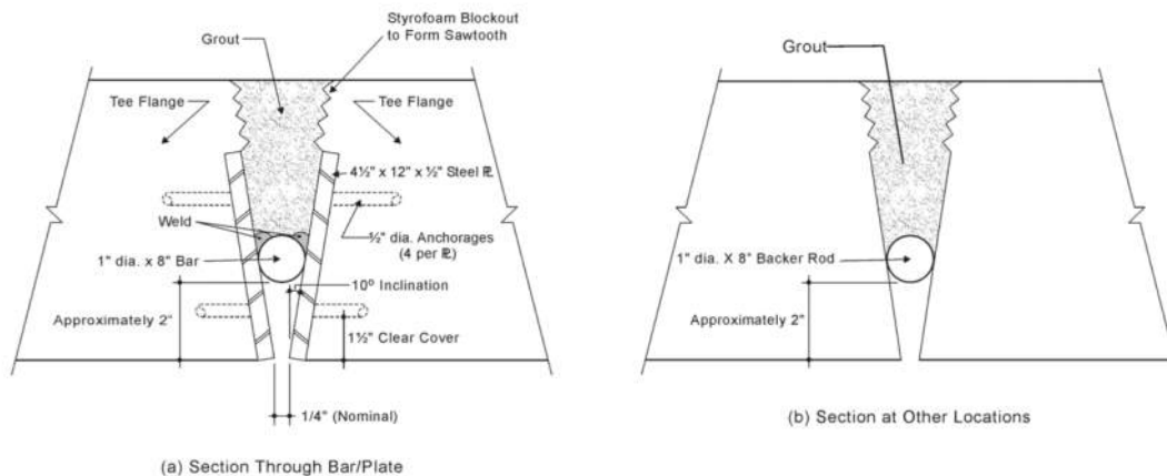
Figure 2.3: New Types of Keyway Details introduced in Texas Study for Double Tee Multibeam Bridges (retrieved from Jones, 2001)
