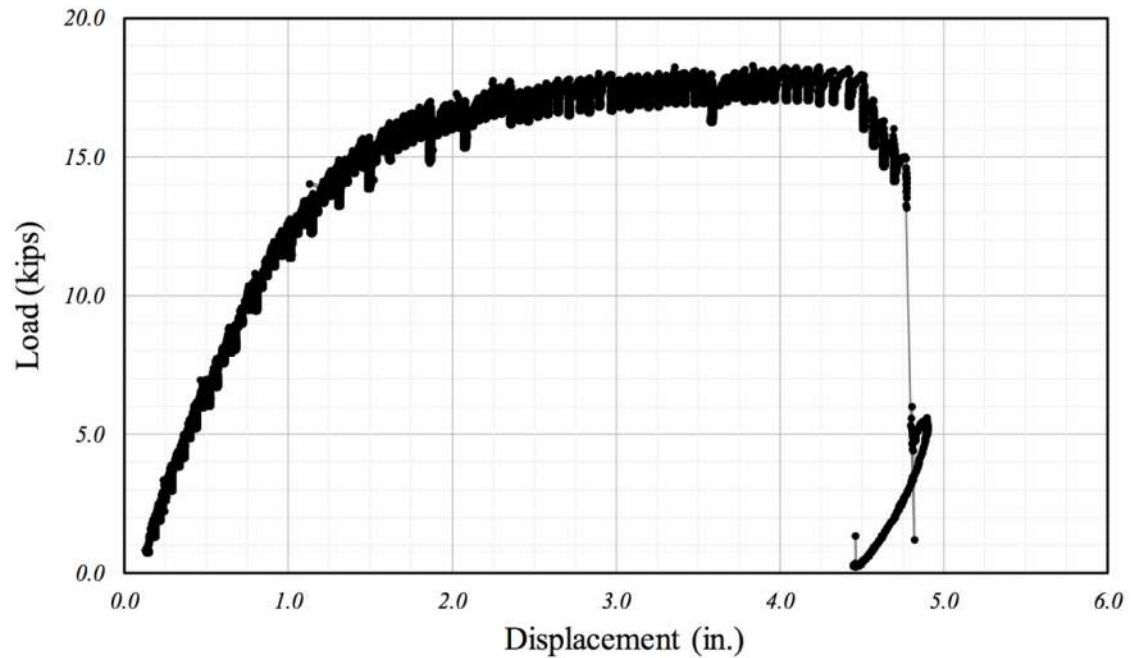
Figure 3.41: Load-Displacement Curve (Specimen F-F-2)
