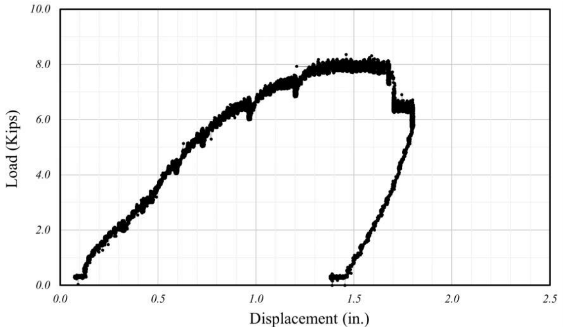
Figure 3.23: Load-Displacement Curve (Specimen C-C-1)
