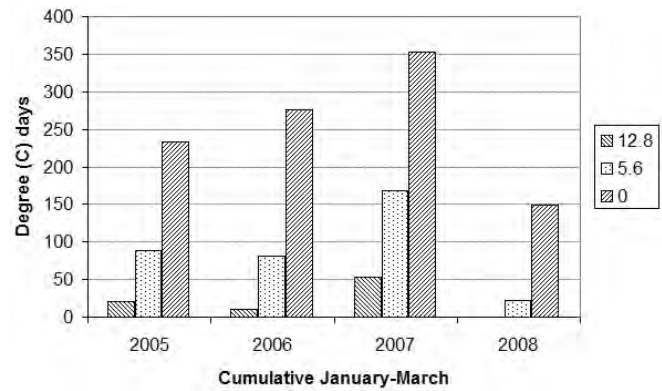
Figure 1. Number of accumulated degree-days above 12.8, 5.6, and 0°C (55, 42, and 32°F) during January-March in years of whooping crane egg production in central Wisconsin, 2005-08 (data from NOAA weather station, Necedah NWR). Note: There were no days with temperatures above 12.8°C during January-March 2008.
