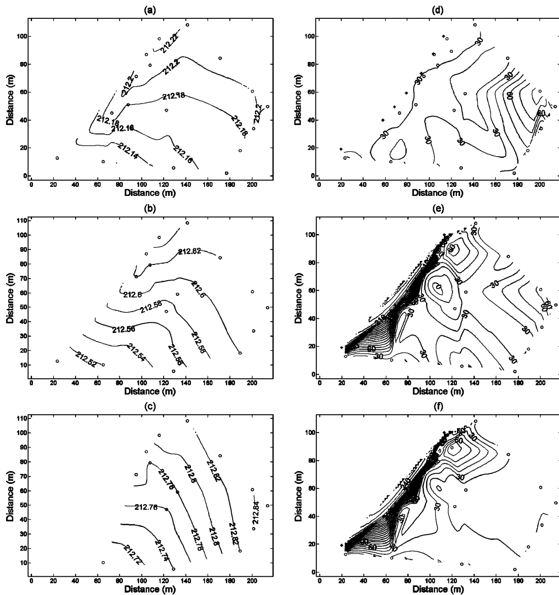
Figure 6. Water table ((a) (c)) and total phosphorus ((d) (f)) concentration ( \mu\text{g}/\text{l} as P) contour plots for the Barren Fork Creek site during the rising limb ((a) (d)) and the recession limb ((b) (e)) of March 23, 2010 high-flow event, and the recession limb ((c) (f)) of March 25, 2010 high-flow event. Interpolations are based on measured data from wells (circles) and the stream (stars). See Table I and Figure 3 for more information on hydrologic conditions at the time of sampling. The loss of observation wells (c) is due to rapid streambank erosion rates (Midgley et al., 2011).
