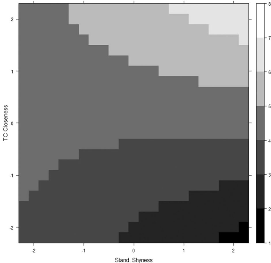
Fig. 3. Predicted surface plot depicting the interaction between child shyness and child-teacher closeness for social competence. Dark grey represents lower predicted social competence scores and light grey represents higher predicted social competence scores.
