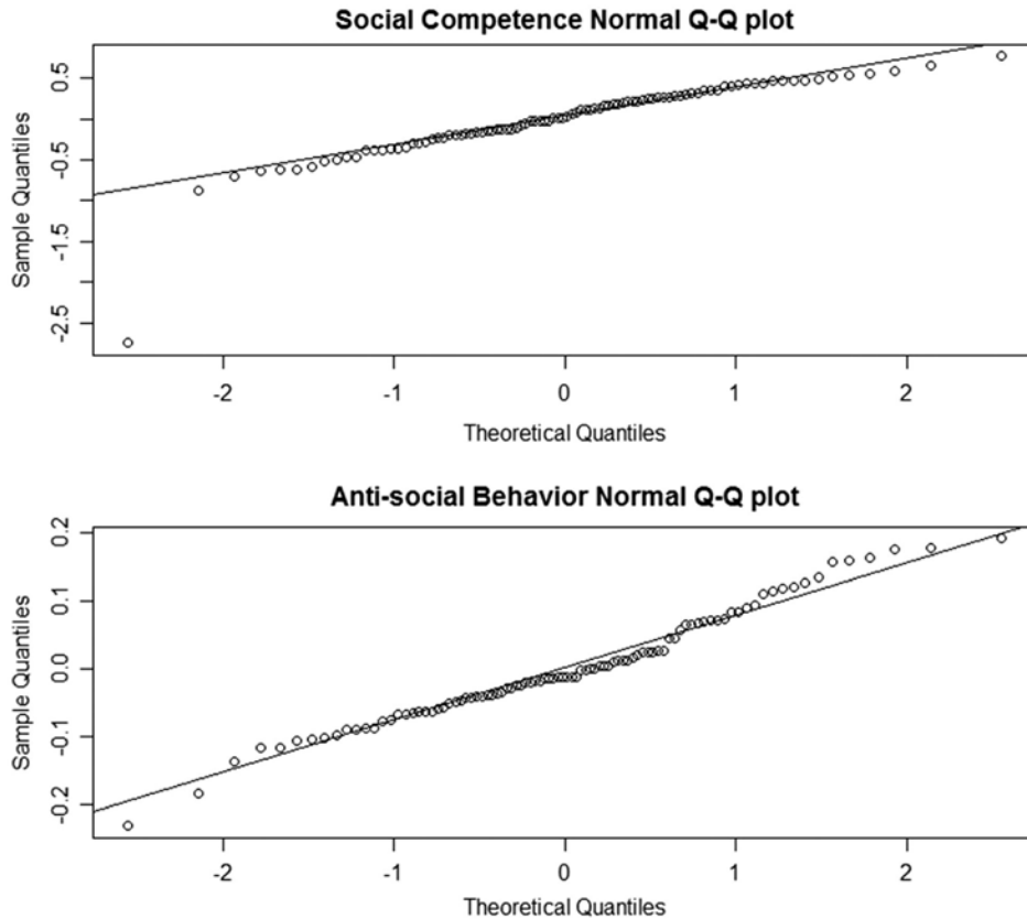
Fig. 2. Normal Q-Q Plots for Teacher-Rated Social Competence and Antisocial Behavior.
