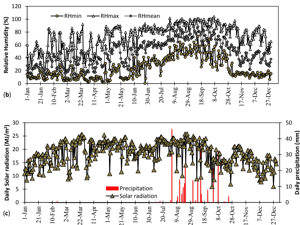
Figure 1. Variation of the (a) daily maximum, minimum and average temperature, (b) daily maximum, minimum and average relative humidity, and (c) daily solar radiation and precipitation from 1 January to 31 December 2015.
