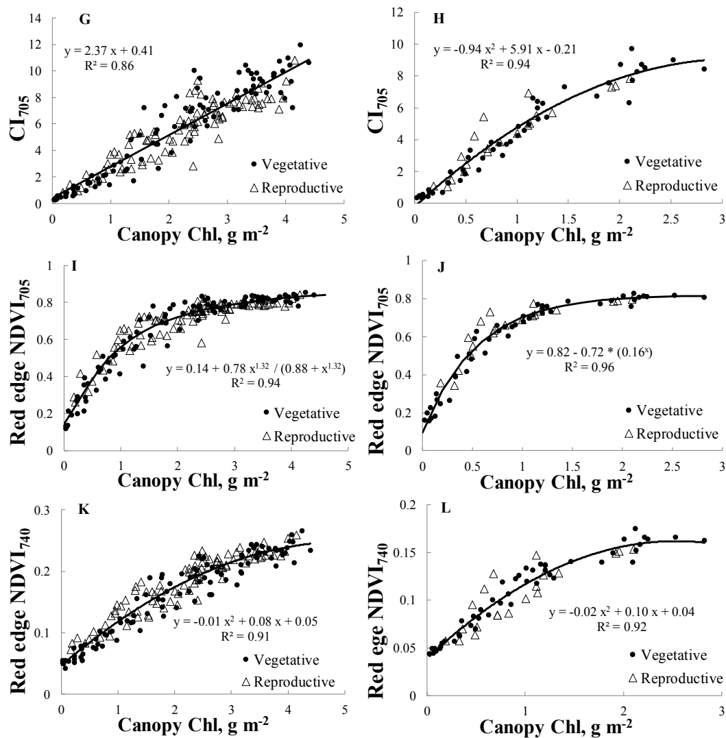
Figure A1. Relationships of VI vs. canopy Chl during both growth stages for SR in maize (A), SR in soybean (B), CI_{green} in maize (C), CI_{green} in soybean (D), green NDVI in maize (E), green NDVI in soybean (F), CI_{705} in maize (G), CI_{705} in soybean (H), red edge NDVI_{705} in maize (I), red edge NDVI_{705} in soybean (J), red edge NDVI_{740} in maize (K) and red edge NDVI_{740} in soybean (L). The solid line represents the best-fit-function of VI vs. canopy Chl developed using samples from the vegetative and reproductive stages combined.
