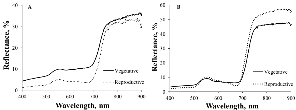
Figure 3. Reflectance spectra of crops with similar canopy Chl in the vegetative and reproductive stages. (A) Maize spectra collected in the vegetative stage (21 June, canopy Chl = 0.98 \text{ g}\cdot\text{m}^{-2} ) and in the reproductive stage (6 September, canopy Chl = 0.99 \text{ g}\cdot\text{m}^{-2} ). (B) Soybean spectra collected in the vegetative stage (8 July, canopy Chl = 0.52 \text{ g}\cdot\text{m}^{-2} ) and in the reproductive stage (12 September, canopy Chl = 0.51 \text{ g}\cdot\text{m}^{-2} ).
