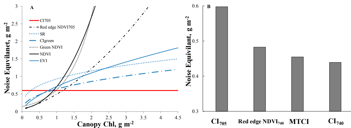
Figure 5. Noise equivalent of canopy Chl estimating in maize and soybean combined by VIs calculated using reflectance simulated at MSI spectral bands for (A) NDVI , green NDVI , red edge NDVI_{705} , SR, EVI, CI_{\text{green}} and CI_{705} and (B) CI_{705} , MTCI, red edge NDVI_{740} and CI_{740} . Note that the maximum noise equivalent (y-axis value) in (A) is five-fold higher than in (B).
