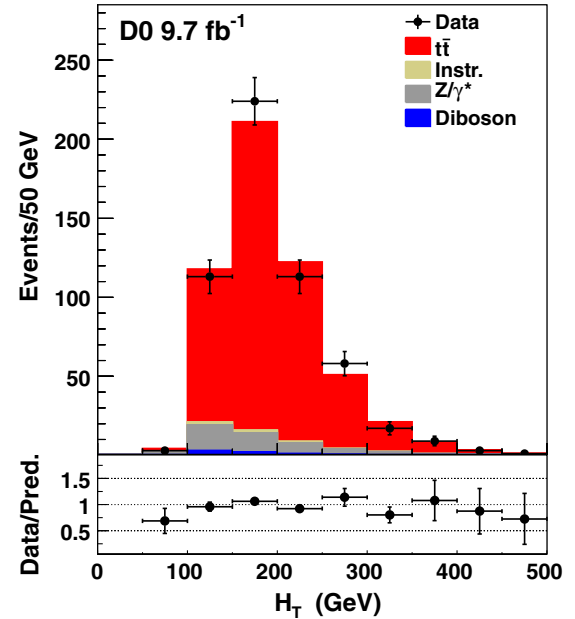
FIG. 4. The distributions in H_T after implementing the k_{\text{JES}} correction, and the ratio of data to the prediction for the combined ee , e\mu , and \mu\mu final states after applying requirements (i)–(vii).
