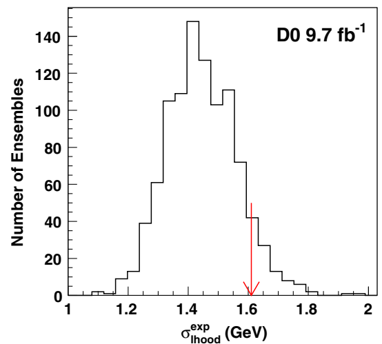
FIG. 7. The distribution in the expected statistical uncertainty \sigma_{\text{lhood}}^{\text{exp}} for the combined ee , e\mu , and \mu\mu channels after applying calibration, for the MC input m_t = 175 GeV. The arrow indicates the statistical uncertainty for data after the calibration ( \sigma_{\text{meas}} ).
