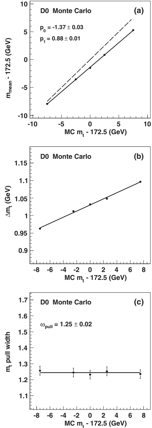
FIG. 5. The response of the ME method in (a) m_t , (b) statistical uncertainty on the m_t , and (c) the pull width, shown as a function of the MC input m_t for the combined ee , e\mu , and \mu\mu channels. The error bars in (a) and (b) are invisibly small. The dashed line in (a) represents the case of ideal response.
