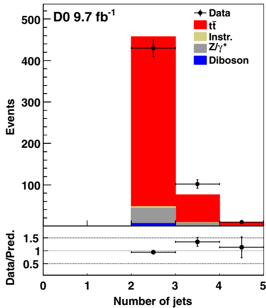
FIG. 2. The distributions in the number of jets and the ratio of data to the prediction for the combined ee , e\mu , and \mu\mu final states after applying requirements (i)–(vii).
