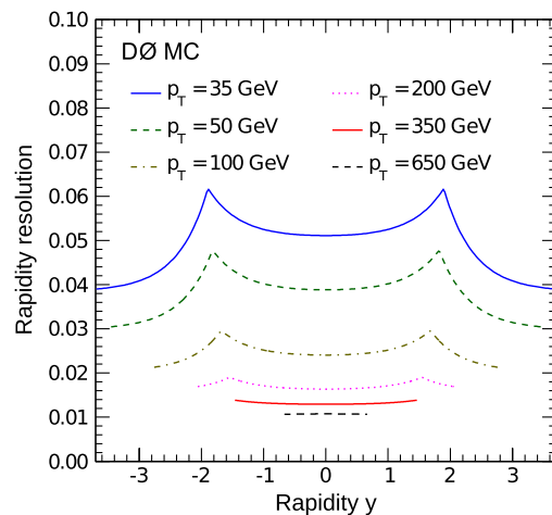
FIG. 33 (color online). (color online) Rapidity resolution (RMS) as a function of y in different jet p_T regions.
