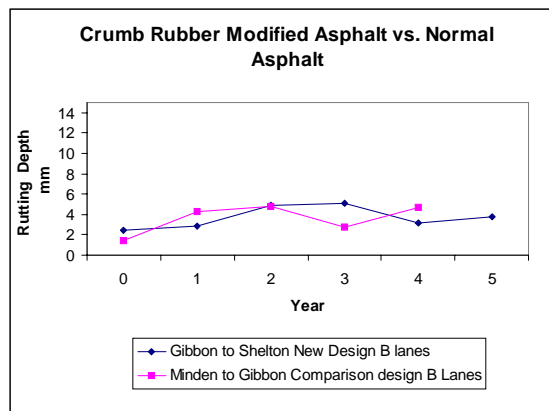
Figure 5.4: Rutting Depth, Gibbon to Shelton and Minden.
