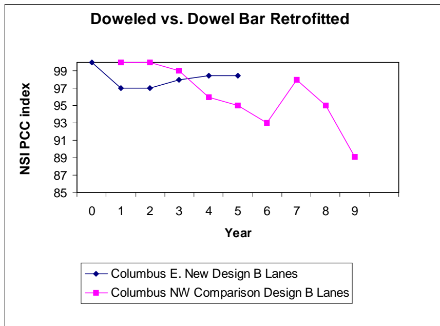
Figure 3.2: NSI PCC, Columbus E. and Columbus NW.
