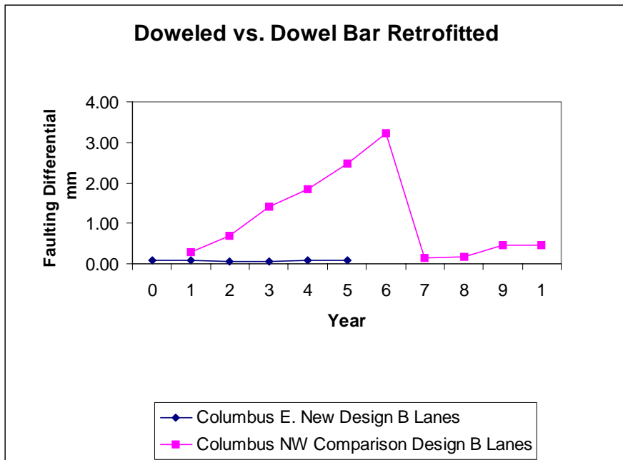
Figure 3.1: Faulting Differential, Columbus E. and Columbus NW.
