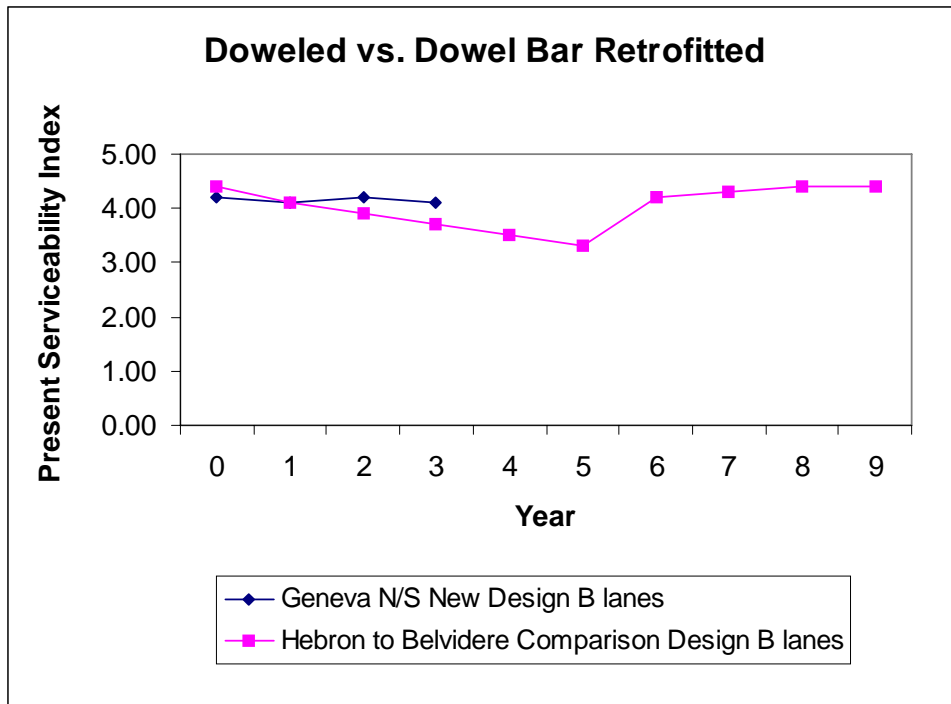
Figure 4.2: PSI, Geneva N/S and Hebron to Belvedere.
