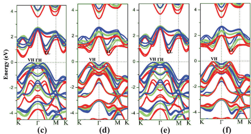
Fig. 5 (a) Atomic structure of two kinds of PtSe 2 bilayers. (b) Band gap of PtSe 2 bilayers versus isotropic strain. Computed band structure of AA stacking bilayers under (c) \epsilon = -8 to 0%, (d) \epsilon = 0 –8% and AB stacking bilayers under (e) \epsilon = -8 to 0%, (f) \epsilon = 0 –8%. The bands with different colors represent the band structures under various strain values, i.e. , blue ( \epsilon = 0\% ), green ( \epsilon = \pm 4\% ) and red ( \epsilon = \pm 8\% ). The Fermi level is located at 0 eV.
