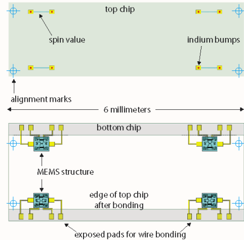
Figure 11. Illustration of the two chips used in the flip chip bonding approach.
