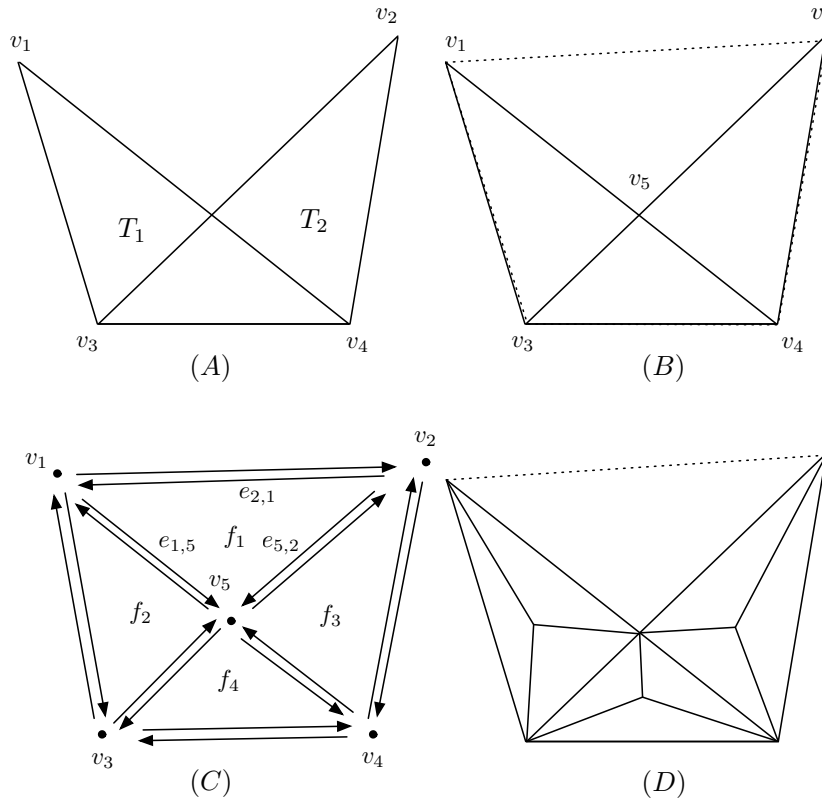
Figure 6. The different steps of Algorithm 1 applied to S = \{T_1, T_2\} . Figure (A) represents the input data. In this example, all boundary segments of all triangles of S contribute to the boundary of S . The line arrangement induced by the carriers of the edges of the input triangles is bounded by the convex hull of the input in (B). A doubly-connected edge list is constructed out of the line arrangement, storing its topological structure in (C). Finally, the triangulation is computed in (D).
