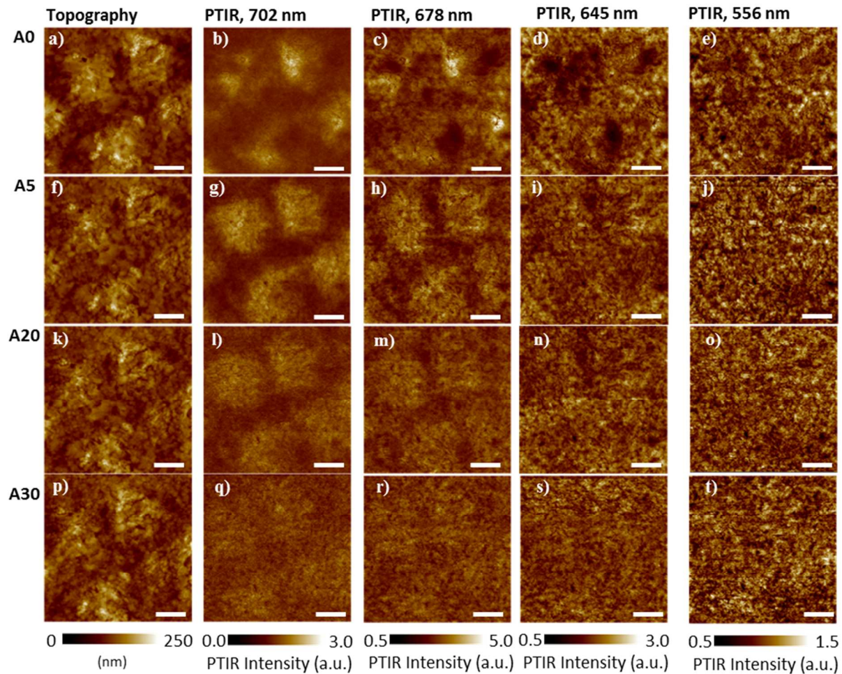
Figure S5. AFM height images (first column) and PTIR maps recorded by illuminating MAPbI 3-x Cl x film at 702 nm (1.77 eV, second column), at 678 nm (1.83 eV, 3rd column), at 645 nm (1.92 eV, fourth column), and at 556 nm (2.23 eV, fifth column). The data are displayed in rows as a function of the annealing: A0 , as prepared sample (first row), A5 , after annealing at 95 °C for 5 min (second row), A20 , after additional annealing at 95 °C for 5 min and at 110 °C for 10 min (third row), and A30 , after additional annealing at 110 °C for 10 min (fourth row). All scale bars are 2.0 μm.
