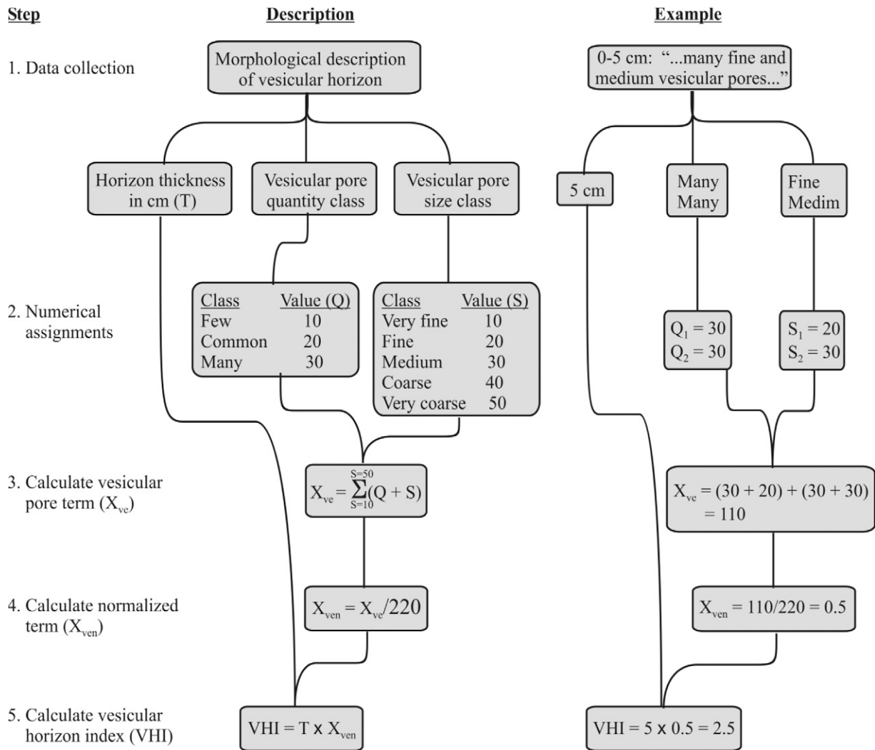
Fig. 7. Outline, description, and example of steps involved in calculation of the vesicular horizon index.
