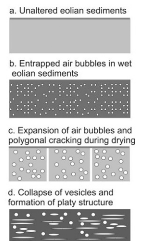
Fig. 3. Summary of processes central to vesicular horizon formation.
