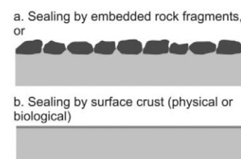
Fig. 3. Summary of processes central to vesicular horizon formation.
