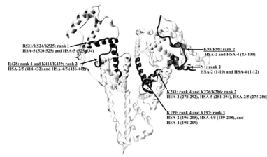
Figure 2. Structure of HSA showing the most likely sites for glycation-related modifications, as based on a semi-quantitative comparison of the data obtained in this study. The regions that were found to have the highest levels of modification are highlighted. The amino acids that contained the highest amounts of modification within these regions are also shown.
