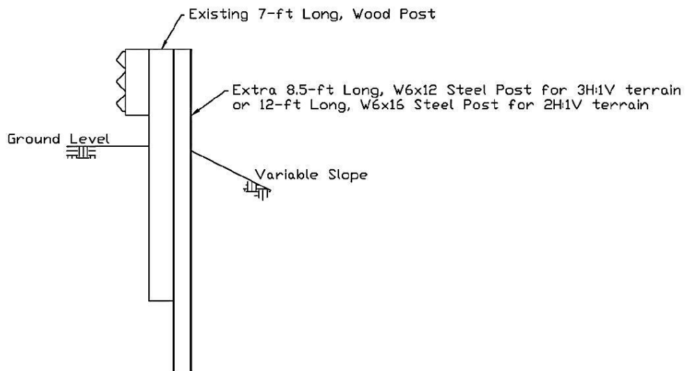
Figure 27. Driven-Post Design [30]
