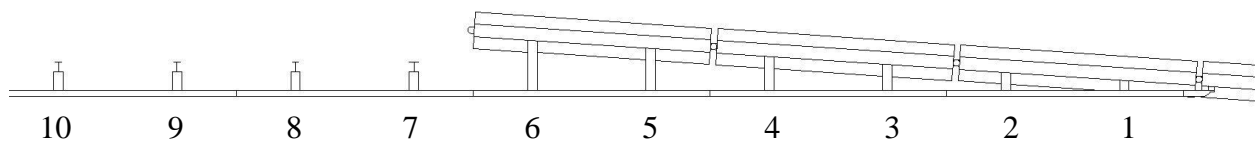
Figure 82. MGS with Fully-Blocked Rail – Impact Locations
