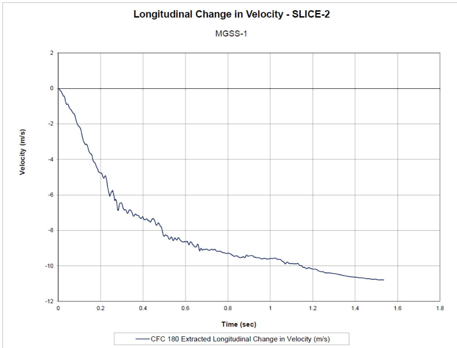
Figure E-10. Longitudinal Occupant Impact Velocity (SLICE-2), Test No. MGSS-1
