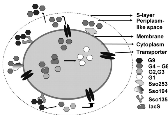
FIG 6 Model illustrating the hydrolysis and transport of cellodextrins in S. solfataricus .
