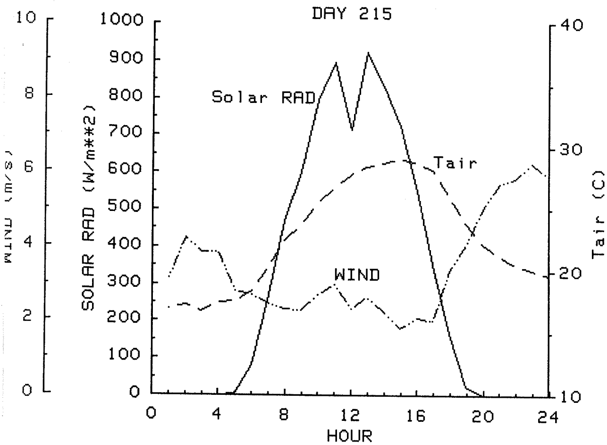
Figure 49. Hourly values of solar radiation, wind speed and air temperature on August 3, 1986 (Day 215).
