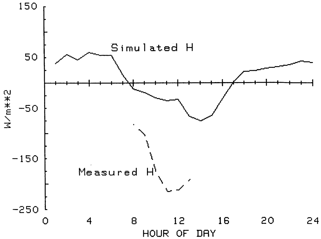
Figure 53. Measured and simulated values of sensible heat flux (H) for August 3, 1986 (Day 215).
