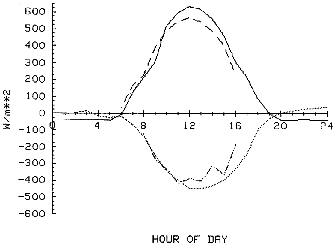
Figure 50. Measured and simulated values of net radiation ( R_n ) and latent heat flux ( LE ) for July 30, 1986 (Day 211).
