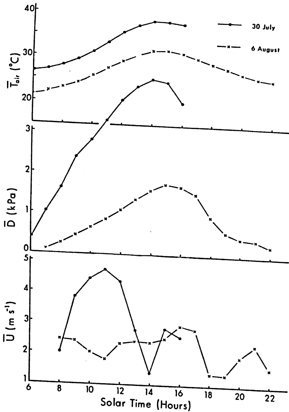
Fig. 31. Diurnal patterns of mean air temperature ( \bar{T} ), mean vapor pressure deficit ( \bar{VPD} ), and mean wind speed ( \bar{U} ) over a tall grass prairie near Manhattan, Kansas. These measurements were made at 1.25 m above ground. 30 July and 6 August 1986.
