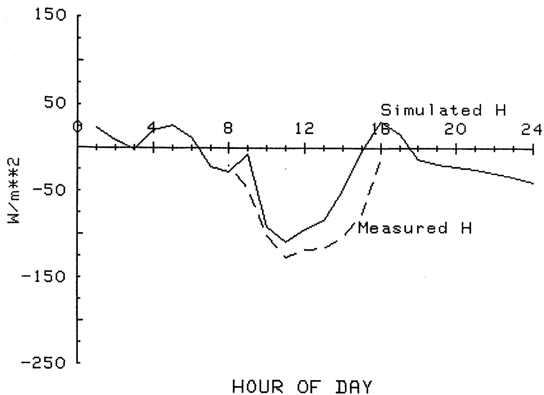
Figure 52. Measured and simulated values of sensible heat flux (H) for July 30, 1986 (Day 211).
