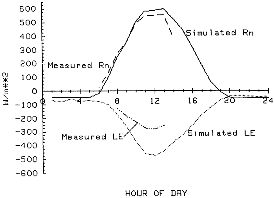
Figure 51. Measured and simulated values of net radiation (Rn) and latent heat flux (LE) for August 3, 1986 (Day 215).
