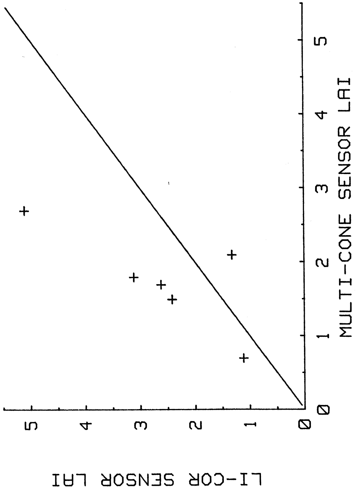
Figure 33. Comparison of estimated LAI values from the multicone sensor with the LI-COR sensor.
