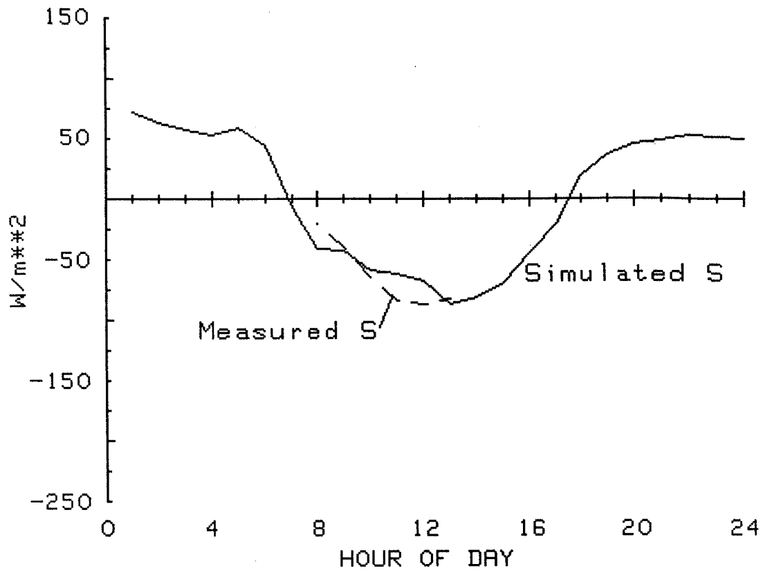
Figure 55. Measured and simulated values of soil heat flux (S) for August 3, 1986 (Day 215).
