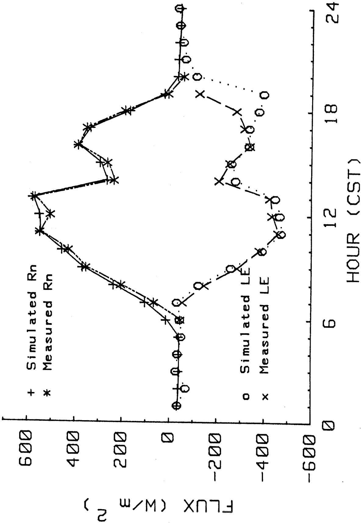
Figure 42. Comparison of measured and simulated Rn and LE fluxes on May 30, 1985 (Day 150).
