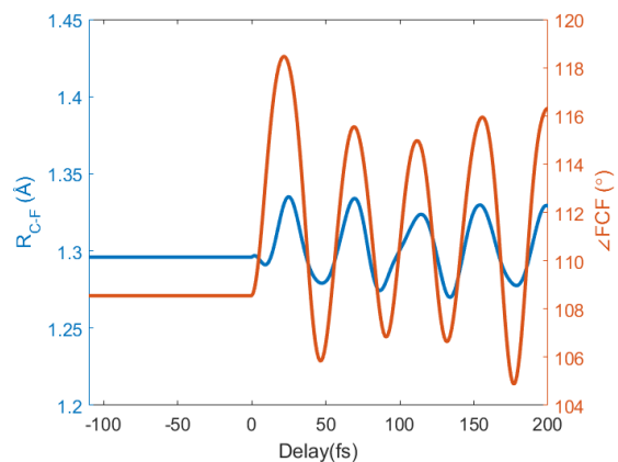
Fig. S6. Simulated structural evolution after one-photon excitation. R C-F and ∠FCF are color-coded as blue and red, respectively. The vertical axes range for length and angle are adjusted to match each other with a 1.33 Å (ground state C-F distance) radius.
