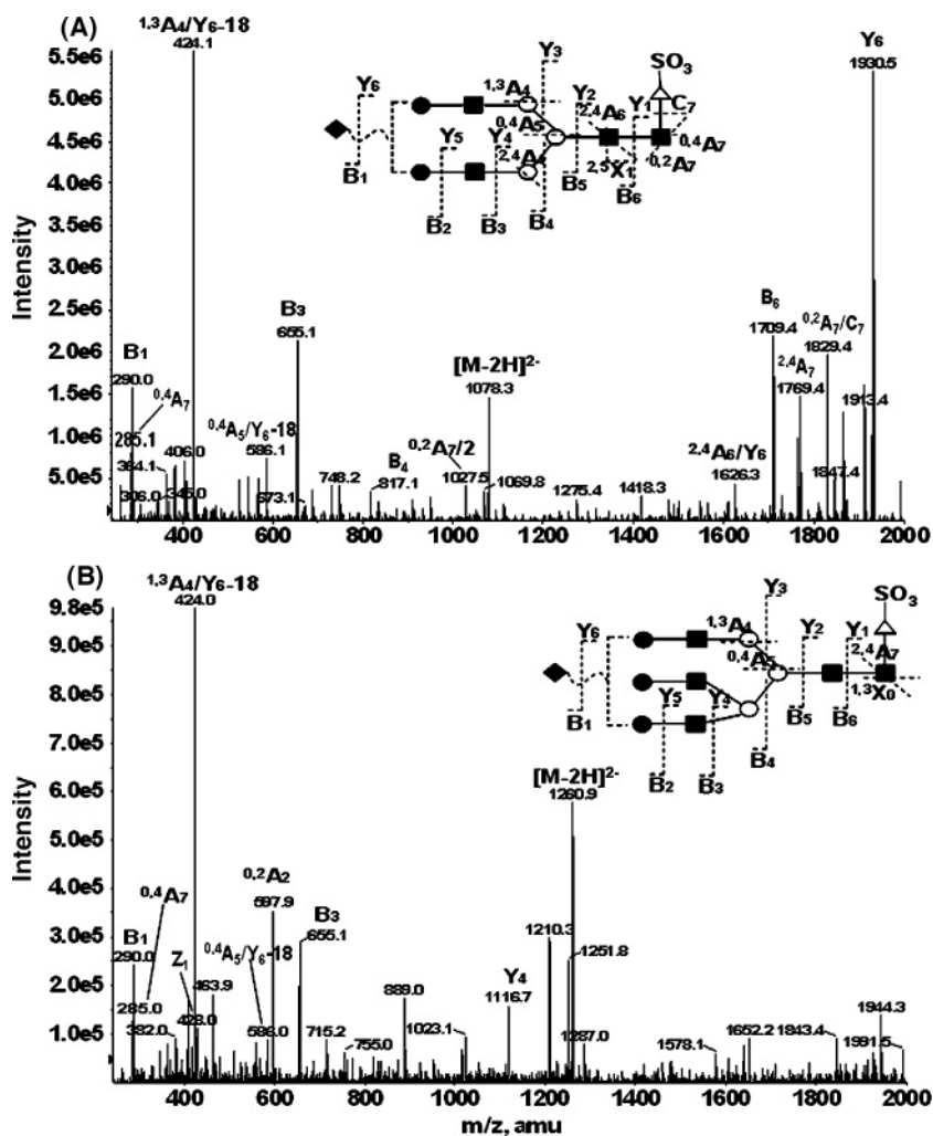
Fig. 5. MS/MS spectra of the putative sulfated N -glycans (A) m/z = 1078 [M-2H]^{2-} and (B) m/z = 1260 [M-2H]^{2-} from tg-FIX (K45 day 45) ( \Delta , fucose; \circ , mannose; \bullet , galactose; \blacksquare , GlcNAc; \blacklozenge , Neu5Ac).
