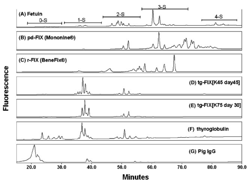
Fig. 2. HPLC N -glycan profiles of (A) Bovine Fetuin, (B) pd-FIX (Mononine ® ), (C) r-FIX (BeneFIX ® ), (D) tg-FIX [K45 day 45], (E) tg-FIX [K75 day 30], (F) porcine thyroglobulin, and (G) pig IgG. The labels 0-S, 1-S, 2-S, 3-S, and 4-S indicate mono-, di-, tri-, and tetrasialylated oligosaccharide groups, respectively.
