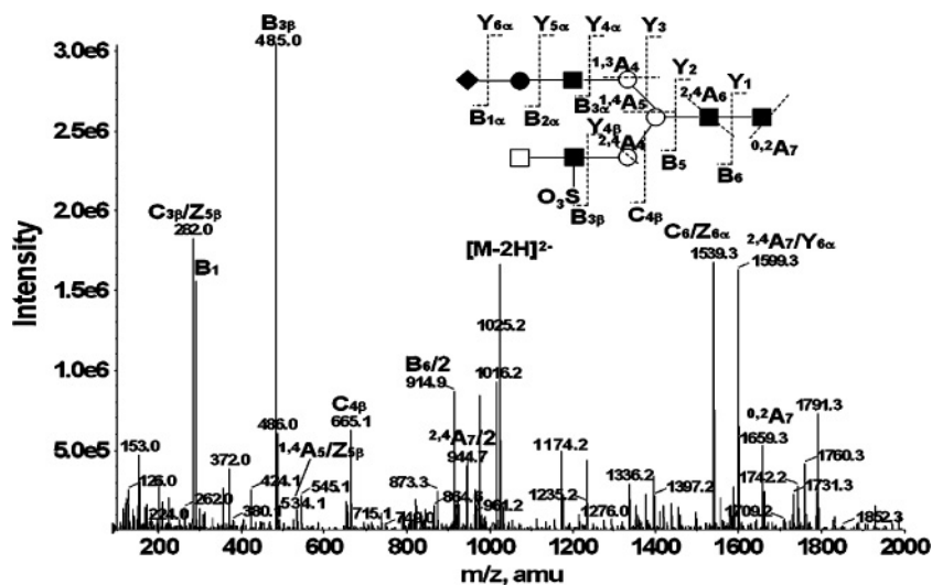
Fig. 6. MS/MS spectrum of the putative sulfated N -glycan ( m/z = 1025 [M-2H]^{2-} ) from tg-FIX (K45 day 45) ( \Delta , fucose; \circ , mannose; \bullet , galactose; \blacksquare , GlcNAc; \square , GalNAc; \blacklozenge , Neu5Ac).
