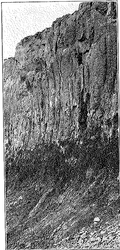
Figure 4. Vertical Section of Deep Subsoil, Loess Above and Drift Below.
