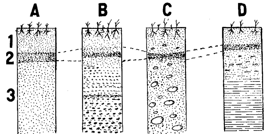
Figure 1. Showing Soil Sections. See Description.
