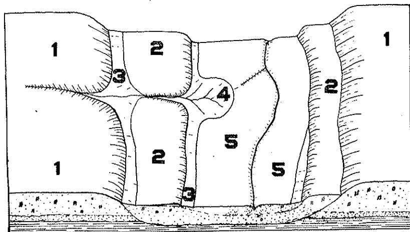
Figure 16. Generalized Cross Section of a Valley, Showing Land Forms.
