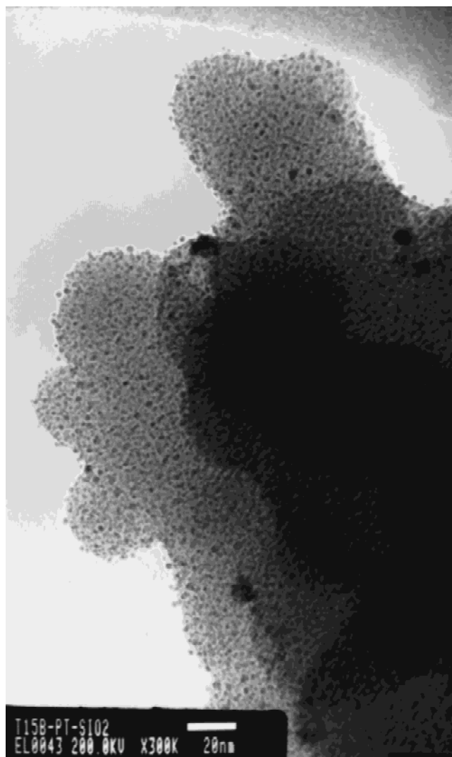
FIG. 8. TEM image of Pt-loaded (calcined) NU-1.
