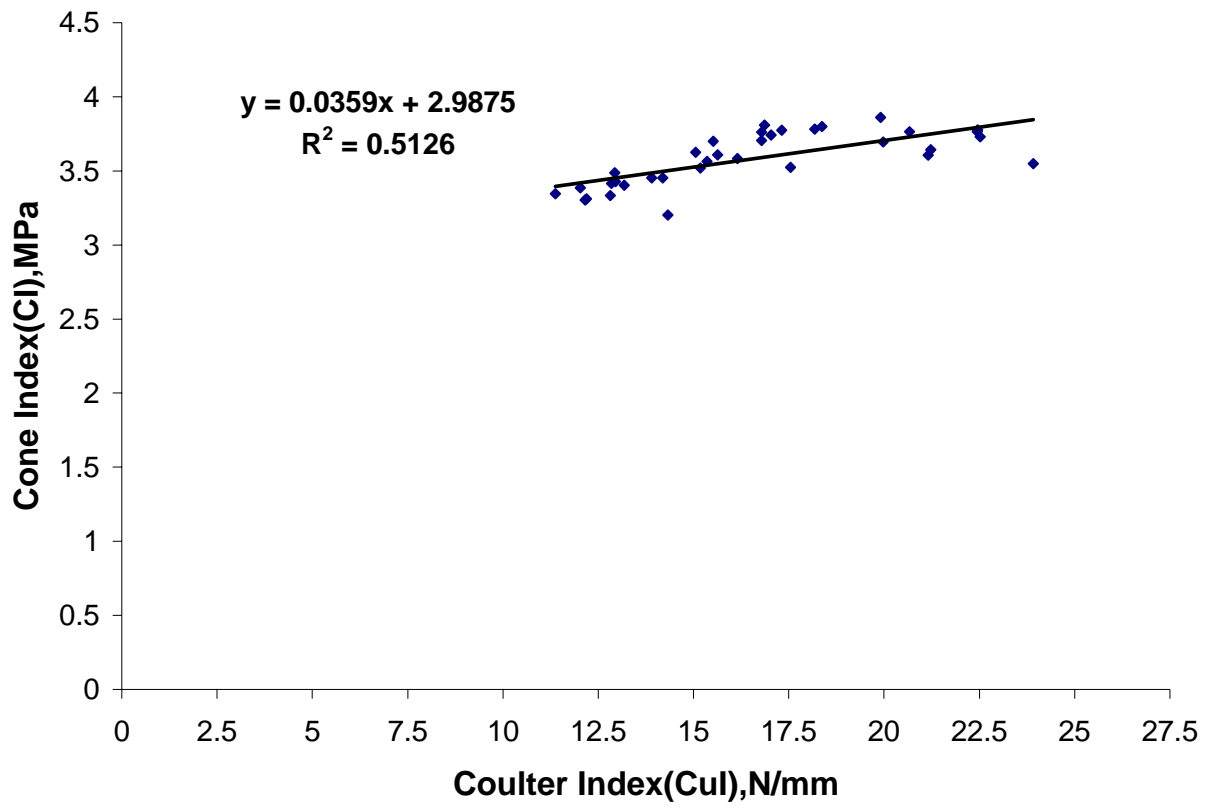
Figure8. Regression analysis between Cul & CI
