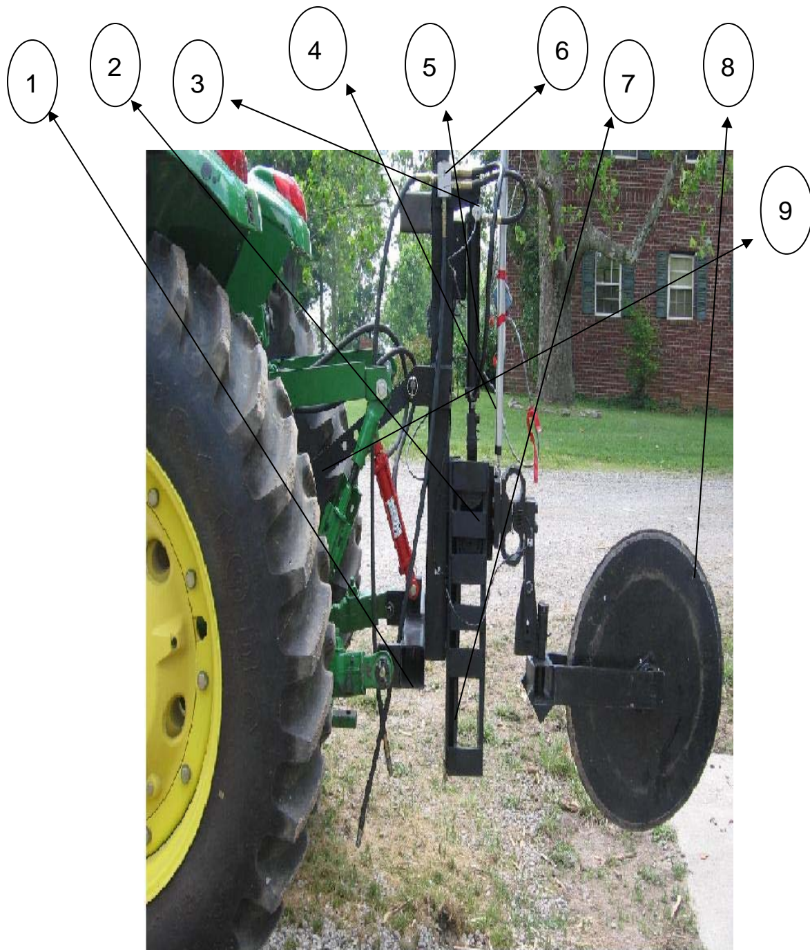
Figure1. Coultter penetrometer mounted on the three-point hitch of a tractor
