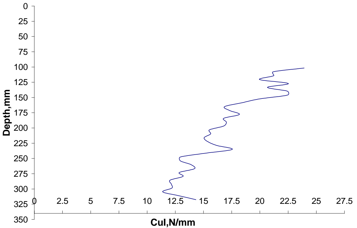
Figure5. Depth Vs average Cul for 0.4ha (one-acre) square grid cell
