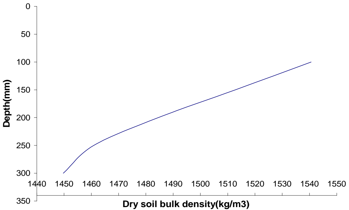
Figure7. Depth Vs average dry soil bulk density for 0.4ha (one-acre) square grid cell
