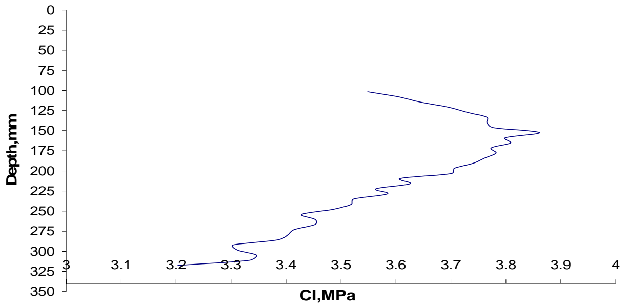
Figure4. Depth Vs average CI for 0.4ha (one-acre) square grid cell
