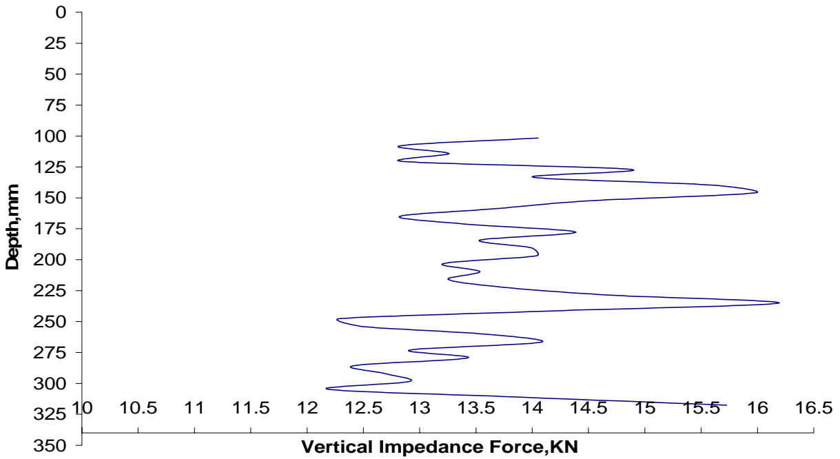
Figure6. Depth Vs average vertical impedance force for 0.4ha (one-acre) square grid cell
